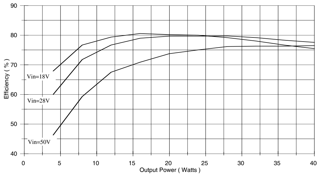
Figure 6. M3G2805S Efficiency
