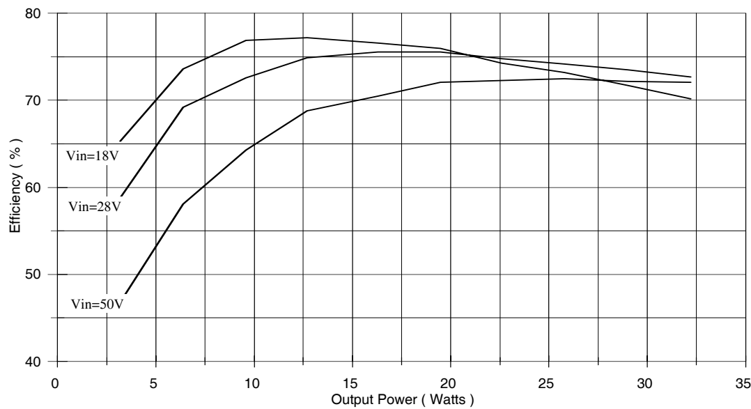
Figure 6. M3G2805S Efficiency
