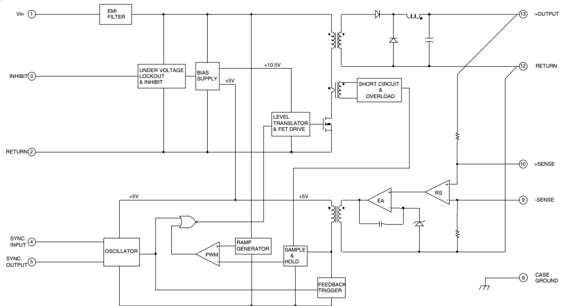
Figure 1. Block Diagram - Single Output
