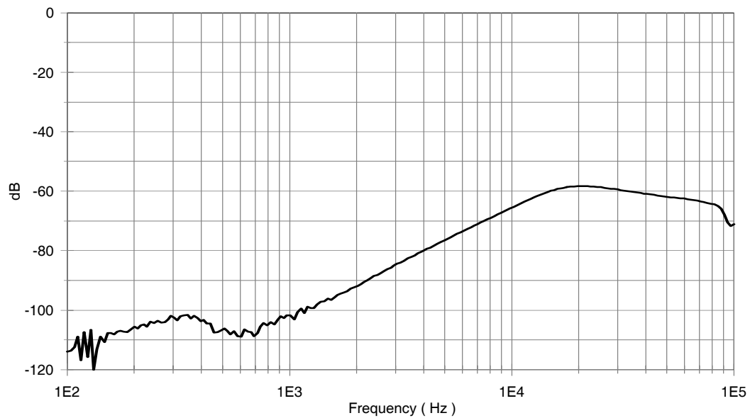
Figure 4. Line Rejection, 28Vdc + 8Vacp-p
