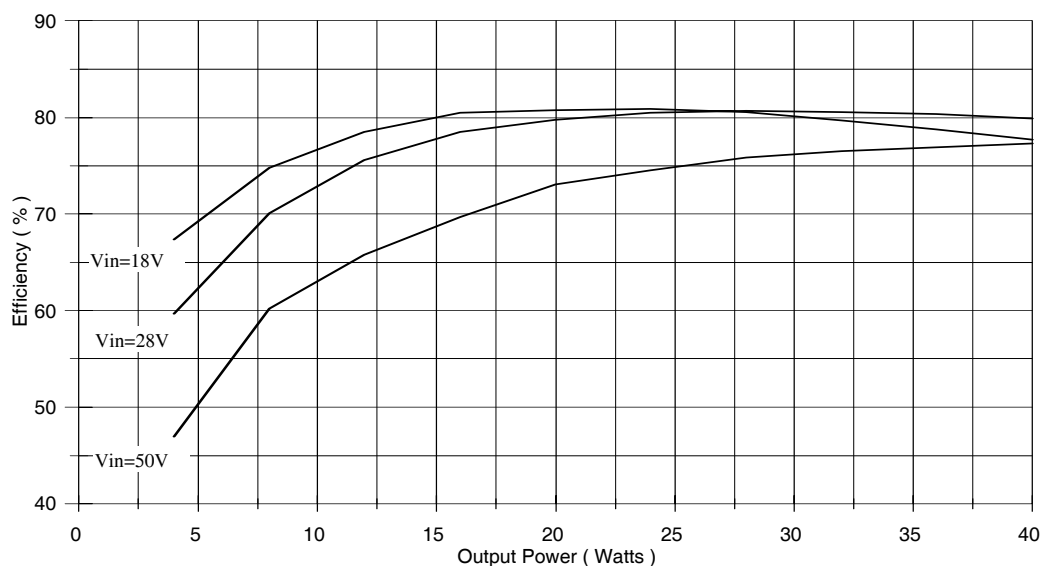
Figure 7. M3G2812S Efficiency
