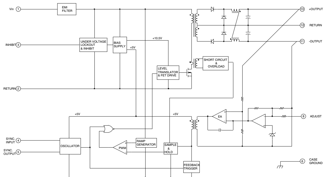
Figure 2. Block Diagram - Dual Output
