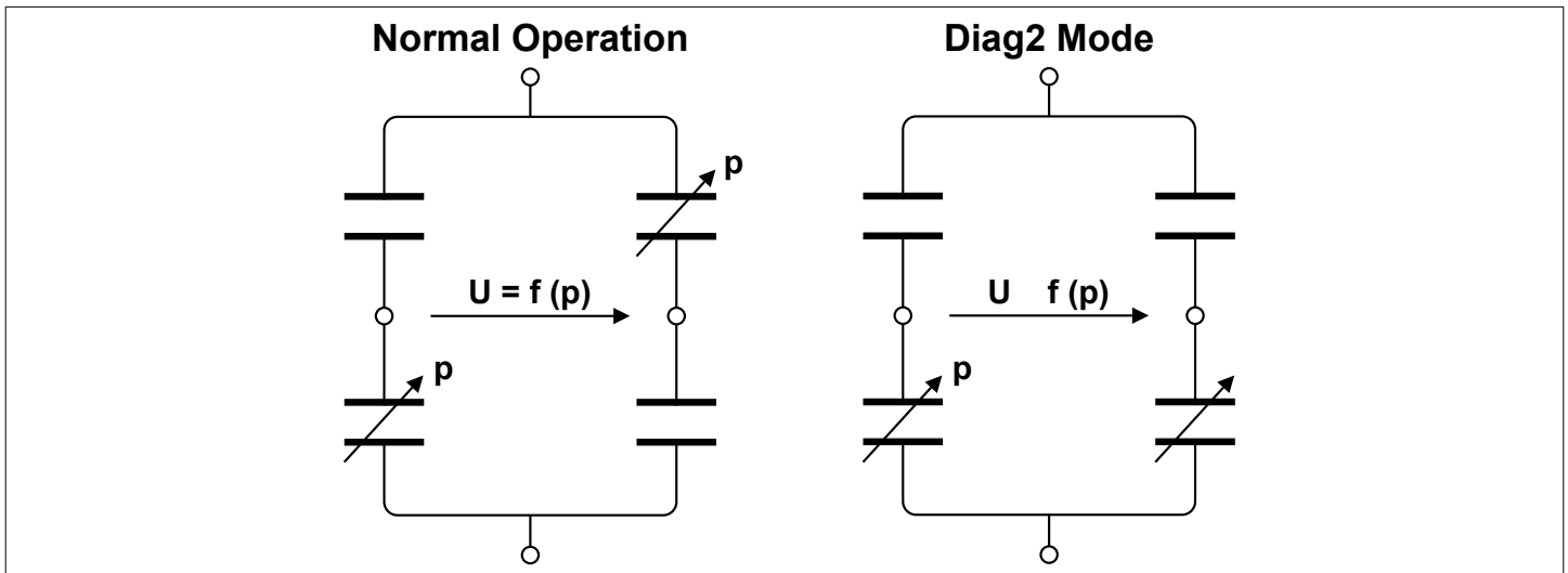
Figure 29 Diag2 functionality
