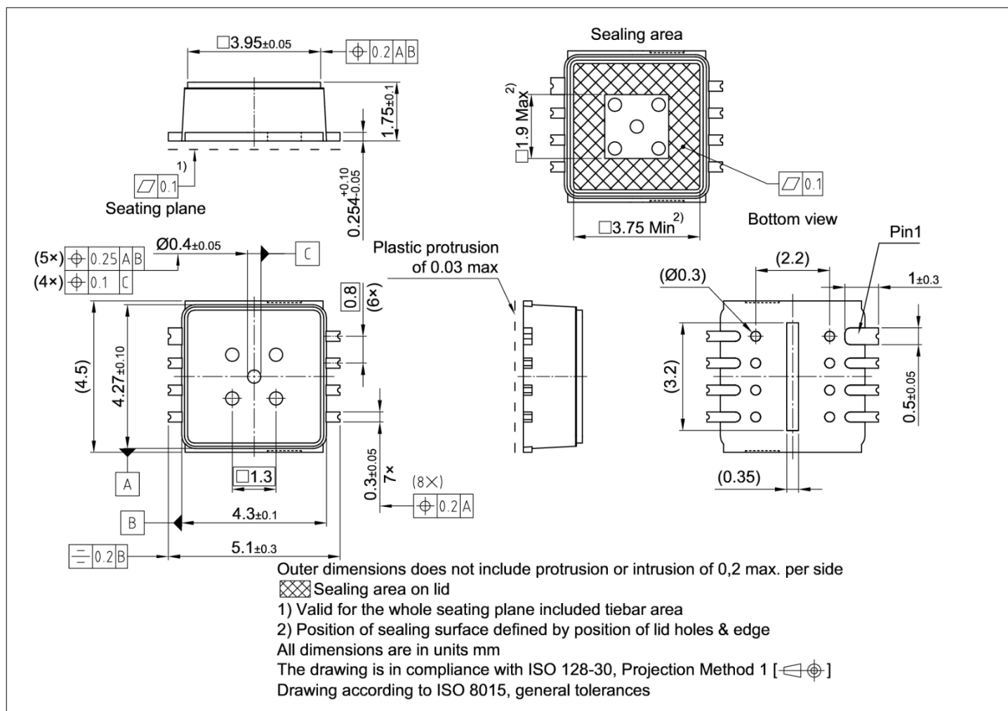
Figure 41 PG-DFN-8-1 outlines
