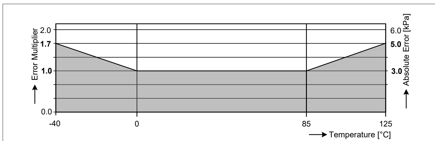
Figure 4 Accuracy for pressure acquisition
