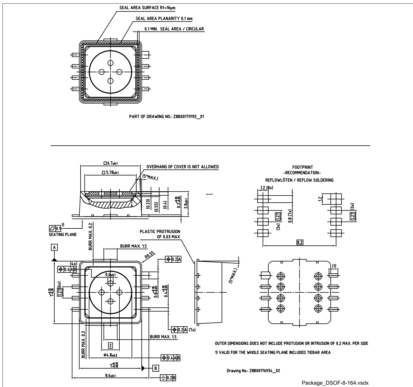
Figure 23 PG-DSOF-8-164 package outline (all dimensions in mm)
