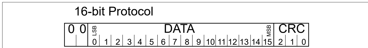
Figure 11 16-bit protocol (21-bit message) in Phase 2 and Phase 3
