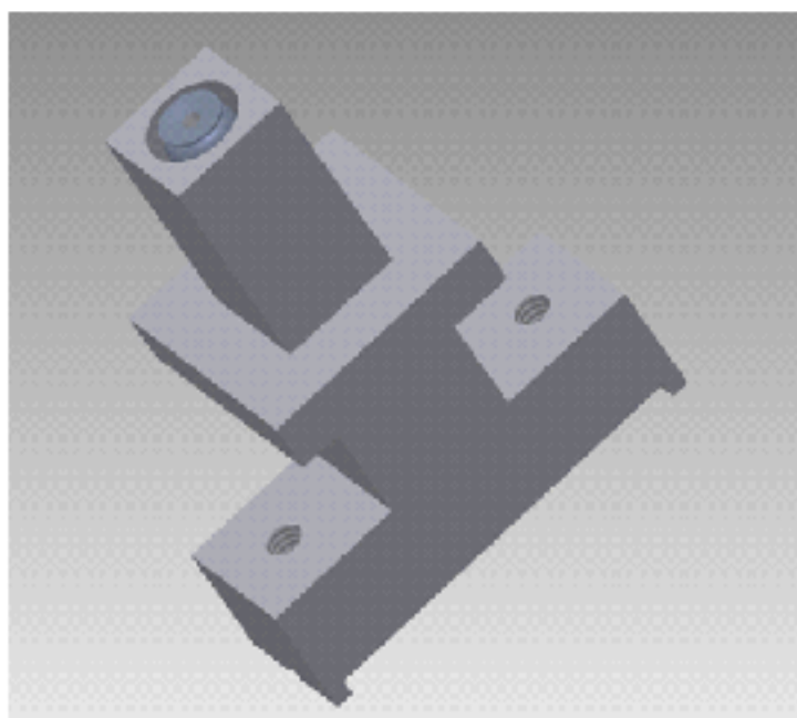
Figure 21 Recommended pick-up nozzle for PG-DSOF package
