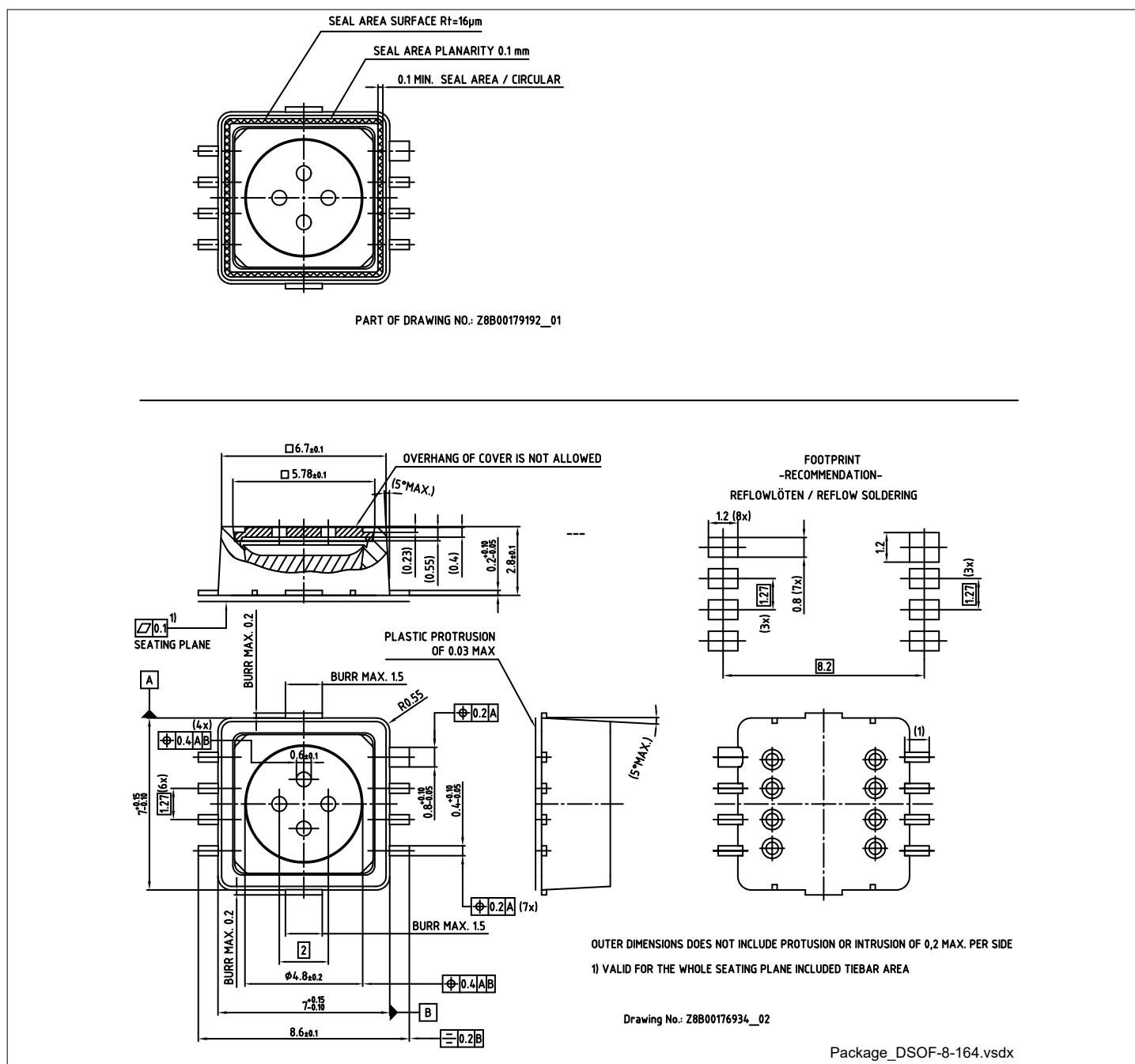
Figure 20 PG-DSOF-8-164 package outline (all dimensions in mm)
