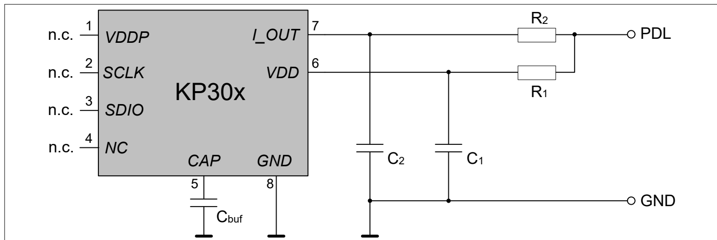
Figure 19 Application circuit example (PG-DSOF-8-164)
