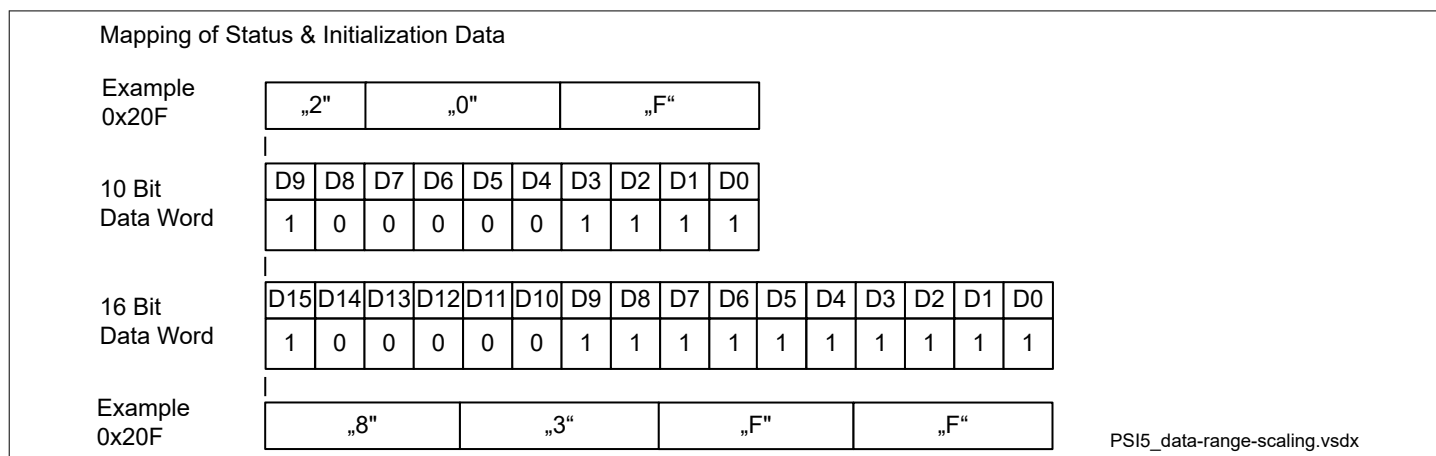
Figure 12 Example: mapping of status and initialization data into a data word
