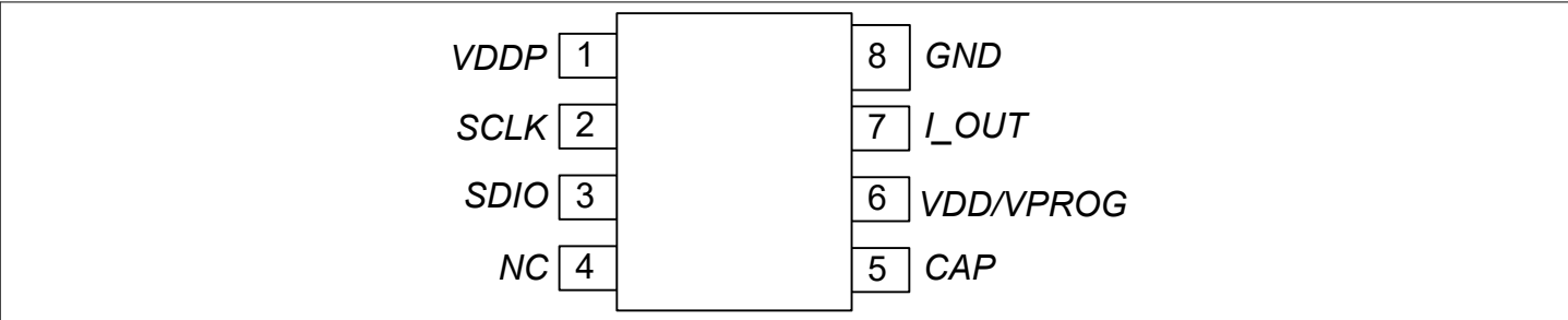
Figure 1 Pin configuration (PG-DSOF-8-164)
