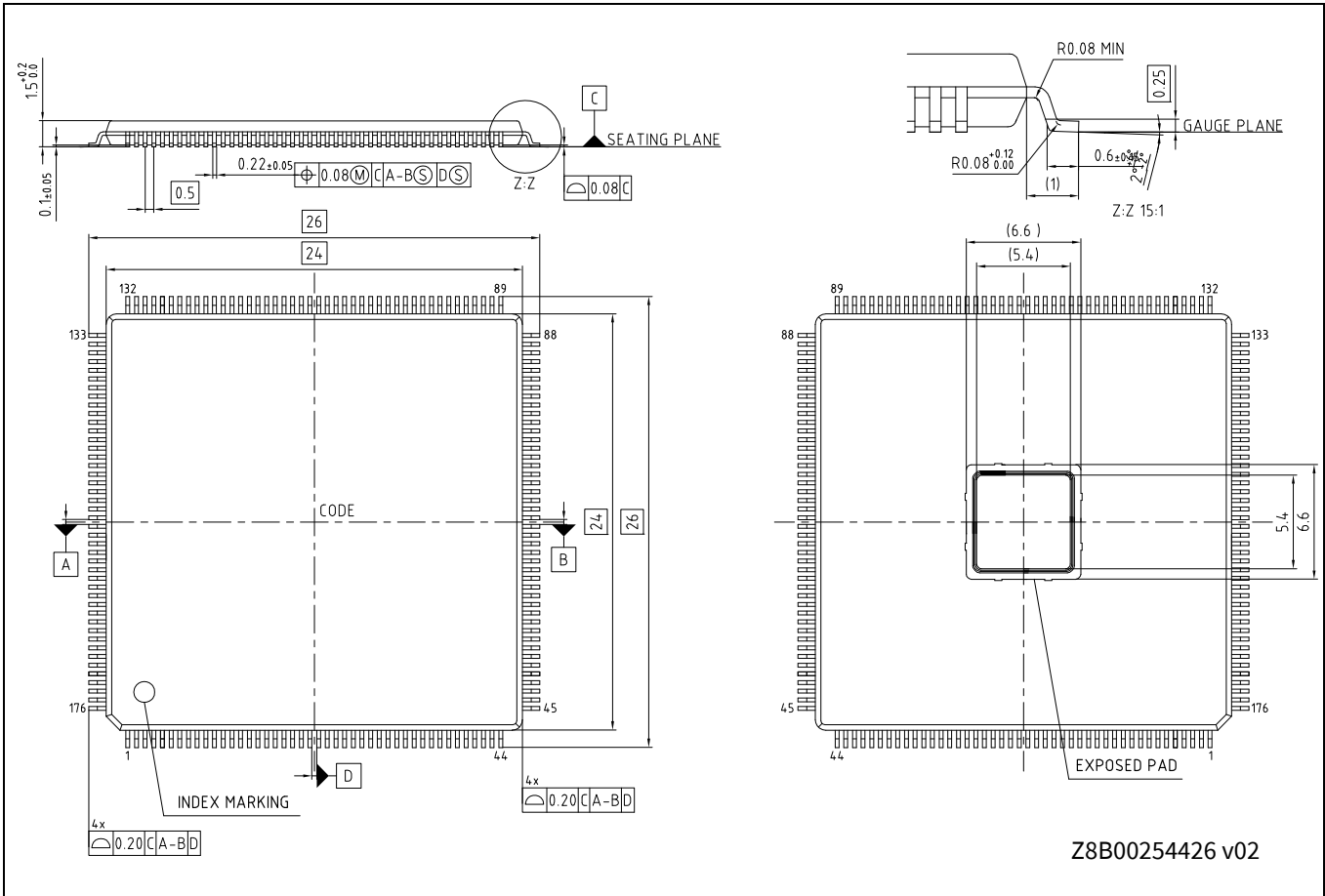
Figure 29-1 Package outline - 176-TEQFP
