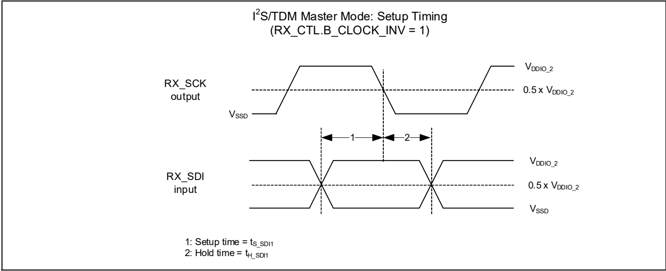
Figure 27-40 Master setup with clock inversion
