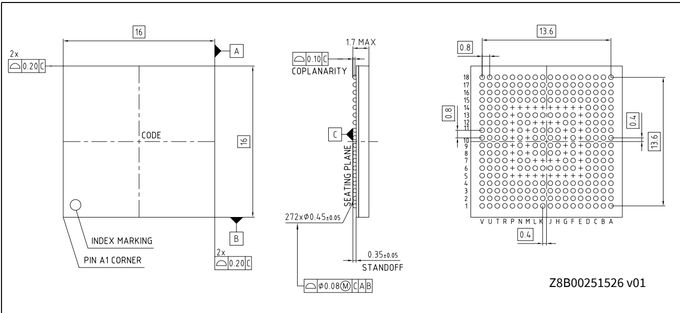
Figure 29-2 Package outline - 272-BGA
