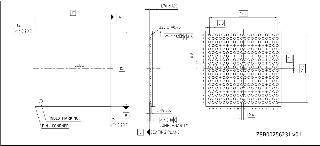
Figure 29-3 Package outline - 320-BGA
