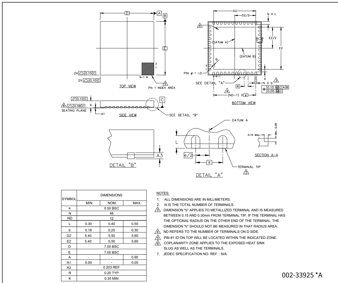
Figure 11 48-pin QFN (7 × 7 × 0.9 mm) package outline, 002-33925
