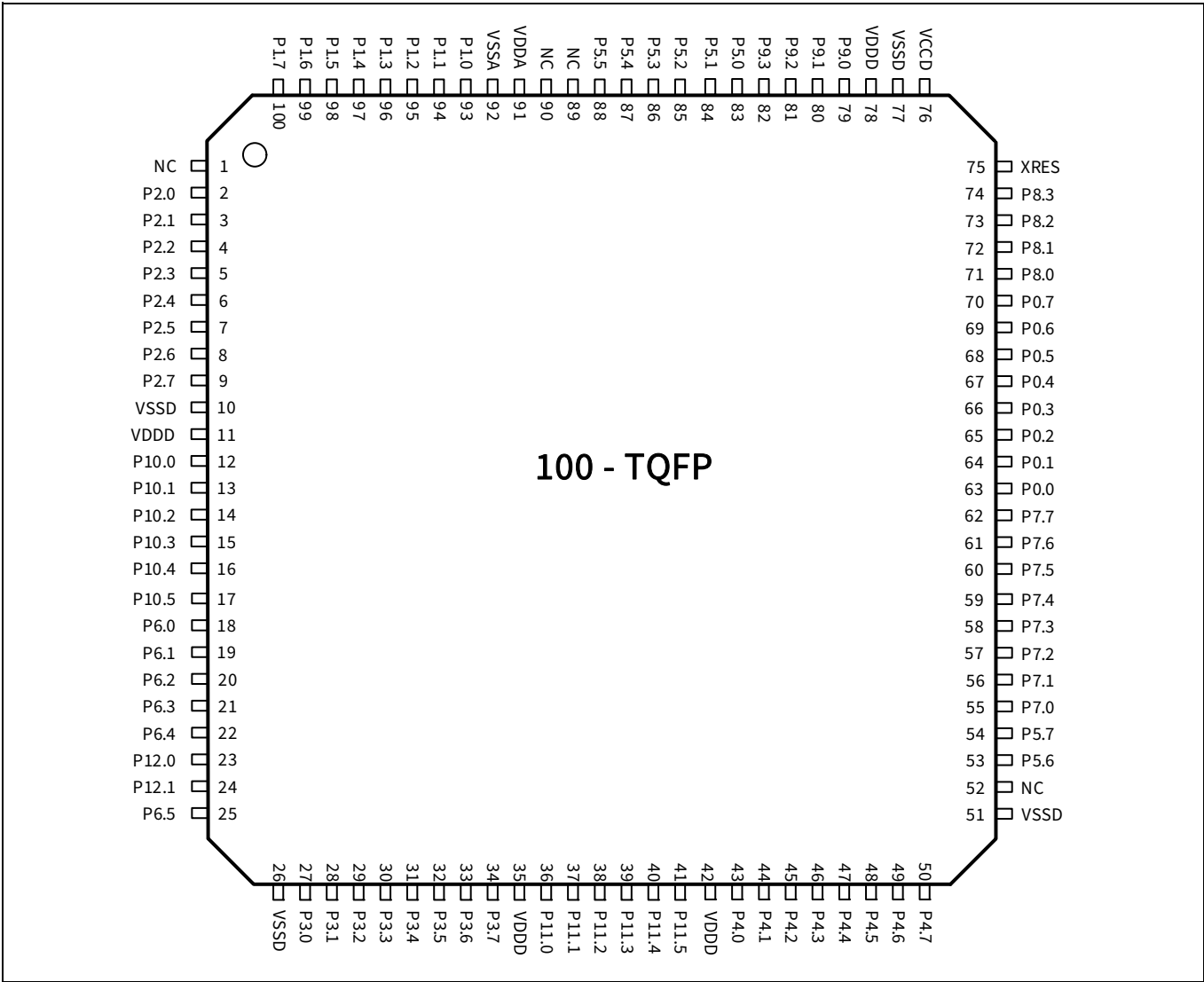
Figure 4 100-TQFP
