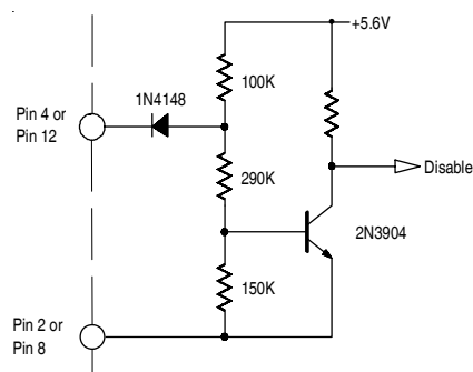
Figure 11. Enable Input Equivalent Circuit
