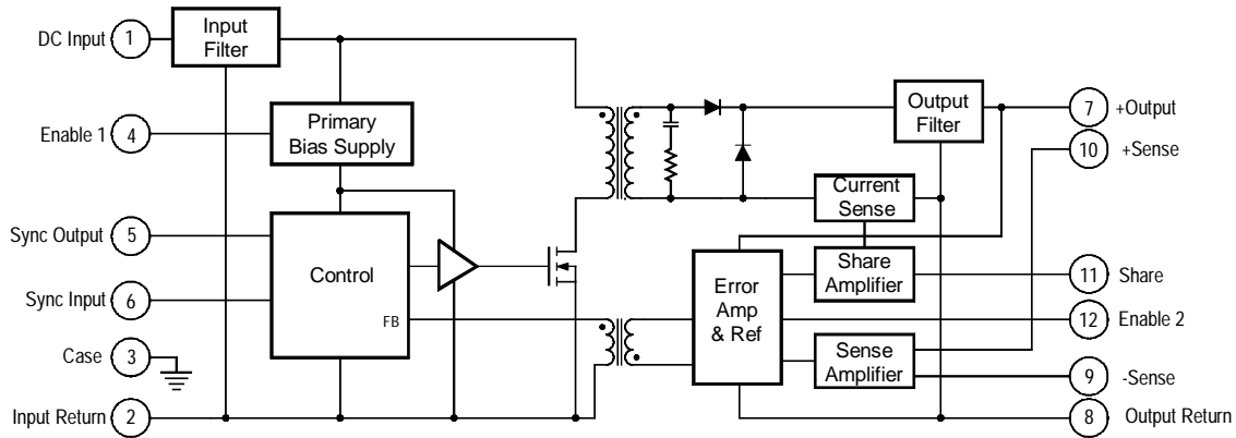
AFL28XXS Circuit Description Figure I. AFL Single Output Block Diagram
