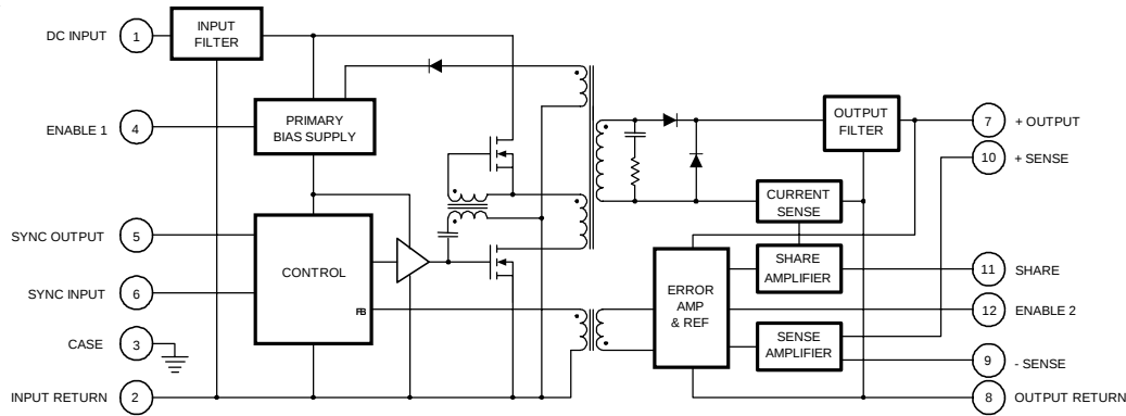
AFL2703R3S Circuit Description Figure I. AFL Single Output Block Diagram
