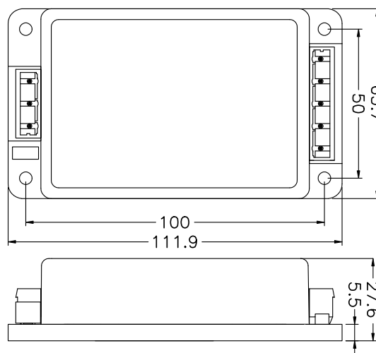
▲ ACE-M804A-P-R10 Dimensions
