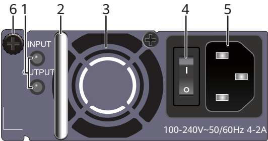
Figure 6-34 Panel of a 250 W AC PoE power module
