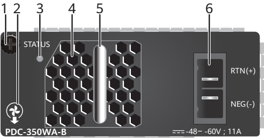
Figure 6-28 Panel of a 350 W DC power module
