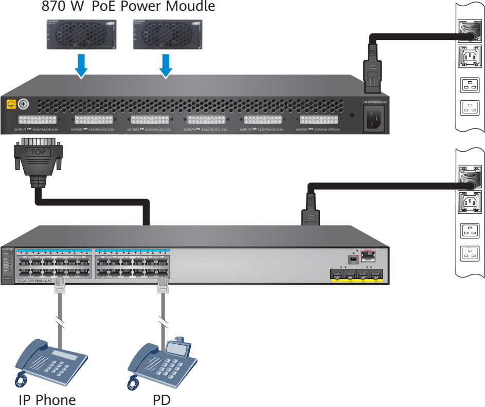
Figure 6-55 PoE power supply for connected switches 870 W PoE Power Moudle
