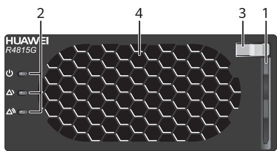
Figure 6-59 Panel of an 870 W PoE power module
