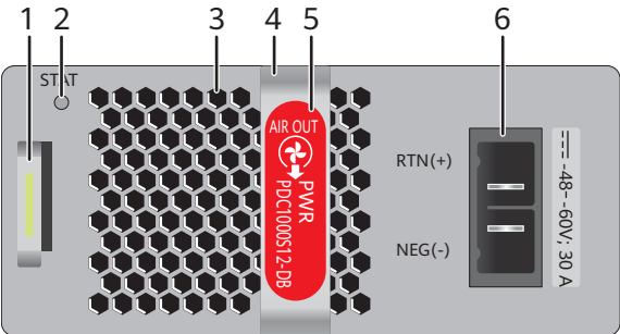
Figure 6-48 Panel of a 1000 W DC power module (PDC1000S12-DB)
