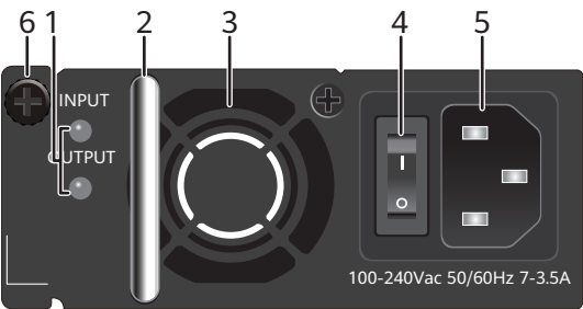
Figure 6-38 Panel of a 500 W AC PoE power module (PAC-500WA-BE)
