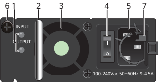
Figure 6-40 Panel of a 580 W AC PoE power module
