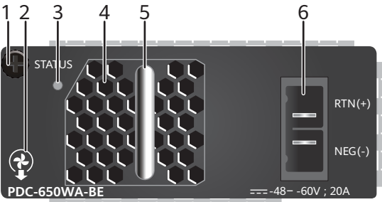
Figure 6-42 Panel of a 650 W DC PoE power module (PDC-650WA-BE)
