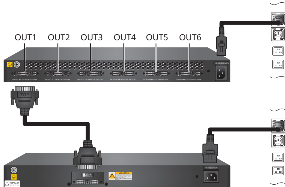
Figure 6-54 Different external power supply systems for RPS1800 and connected switches
