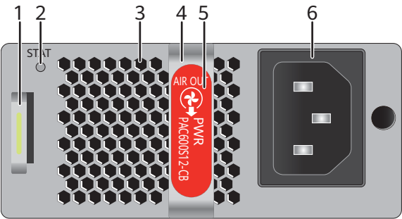
Figure 6-32 Panel of a 600 W AC power module (PAC600S12-CB)
