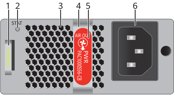
Figure 6-46 Panel of a 1000 W AC PoE power module (PAC1000S56-CB)
