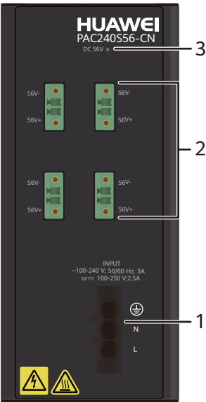
Figure 6-22 Panel of a 240 W AC power module
