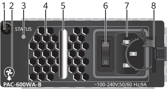
Figure 6-30 Panel of a 600 W AC power module
