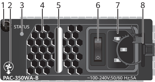
Figure 6-26 Panel of a 350 W AC power module
