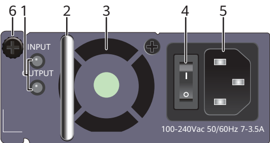
Figure 6-37 Panel of a 500 W AC PoE power module (W0PSA5000)
