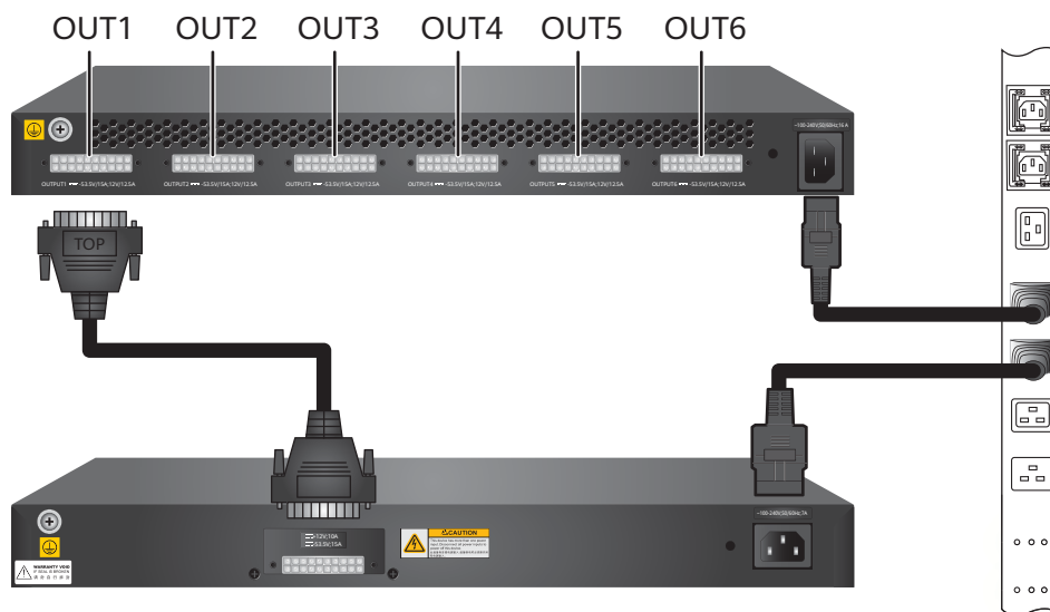
Figure 6-53 Same external power supply system for RPS1800 and connected switches
