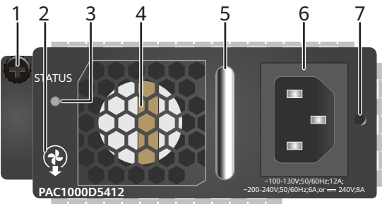
Figure 6-44 Panel of a 1000 W AC PoE power module
