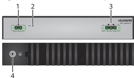
Figure 6-24 Panel of a 260 W AC power module
