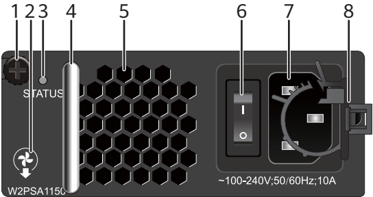
Figure 6-51 Panel of a 1150 W AC PoE power module (W2PSA1150)
