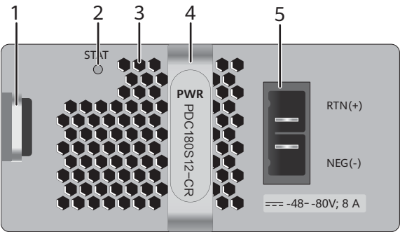
Figure 6-20 Panel of a 180 W DC power module (PDC180S12-CR)
