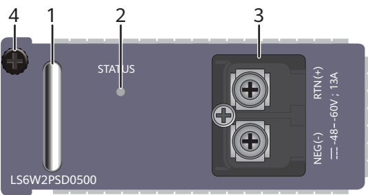
Figure 6-16 Panel of a 500 W DC power module
