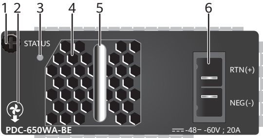
Figure 6-26 Panel of a 650 W DC PoE power module (PDC-650WA-BE)
