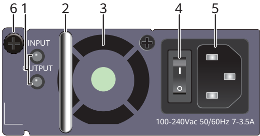
Figure 6-22 Panel of a 500 W AC power module (W0PSA5000)
