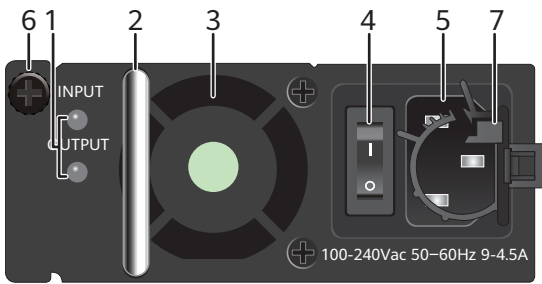
Figure 6-24 Panel of a 580 W AC PoE power module
