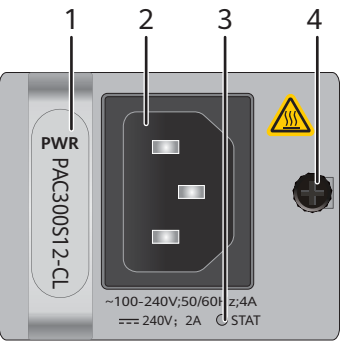
Figure 6-12 Panel of a 300 W AC power module (PAC300S12-CL)
