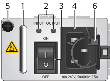
Figure 6-6 Panel of a 170 W AC power module
