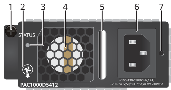
Figure 6-28 Panel of a 1000 W AC PoE power module
