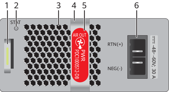
Figure 6-30 Panel of a 1000 W DC power module (PDC1000S12-DB)
