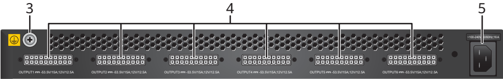
Figure 6-39 Rear view of an RPS1800 power supply
