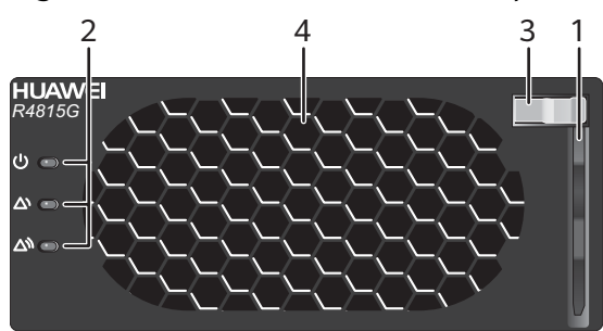
Figure 6-41 Panel of an 870 W PoE power module
