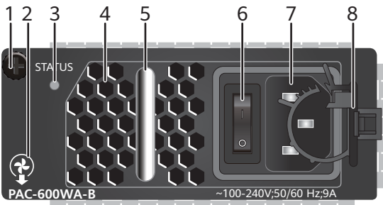
Figure 6-18 Panel of a 600 W AC power module
