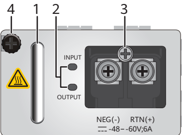
Figure 6-8 Panel of a 170 W DC power module
