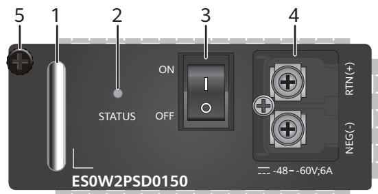
Figure 6-4 Panel of a 150 W DC power module (ES0W2PSD0150)
