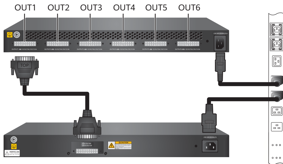
Figure 6-35 Same external power supply system for RPS1800 and connected switches
