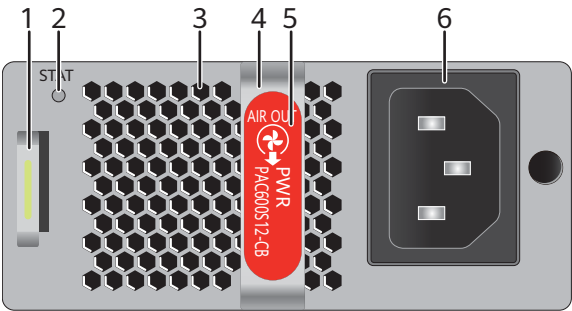
Figure 6-20 Panel of a 600 W AC power module (PAC600S12-CB)
