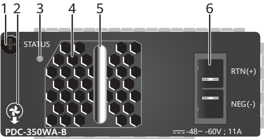
Figure 6-14 Panel of a 350 W DC power module
