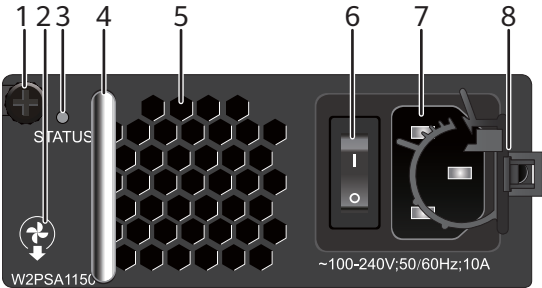
Figure 6-33 Panel of a 1150 W AC PoE power module (W2PSA1150)
