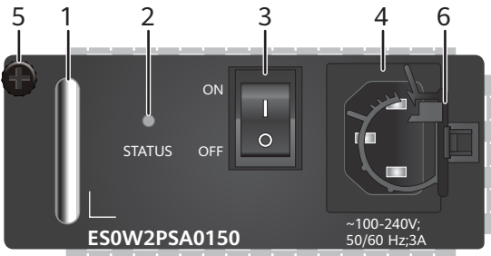
Figure 6-2 Panel of a 150 W AC power module (ES0W2PSA0150)
