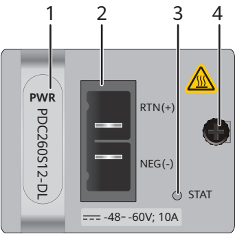
Figure 6-10 Panel of a 260 W DC power module (PDC260S12-DL)
