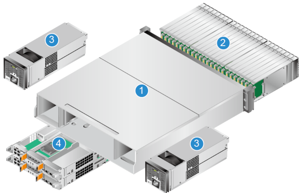
Figure 2-1 Overall structure of a 2 U 25-disk controller enclosure
