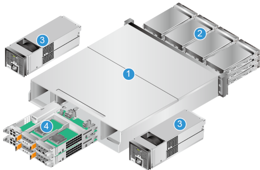
Figure 2-2 Overall structure of a 2 U 12-disk controller enclosure
