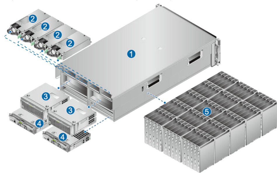
Figure 2-5 Overall structure of a high-density disk enclosure
