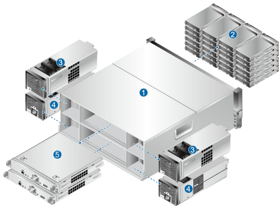
Figure 2-4 Overall structure of a 4 U disk enclosure
