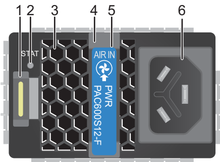
Figure 3-24 PAC600S12-F panel
