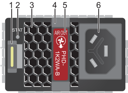
Figure 3-55 PHD-1K2WA-B panel
