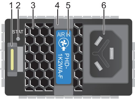
Figure 3-56 PHD-1K2WA-F panel
