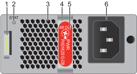
Figure 3-58 Panel of the PHD1K2S12-DB power module
