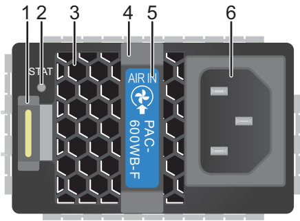
Figure 3-28 PAC-600WB-F panel
