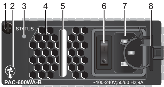
Figure 3-19 PAC-600WA-B panel
