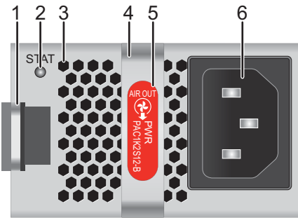
Figure 3-52 PAC1K2S12-B panel
