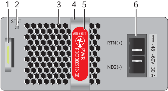
Figure 3-43 Panel of the PDC1000S12-DB power module
