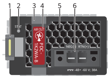
Figure 3-61 Panel of a PDC-1K2WA-B DC power module
