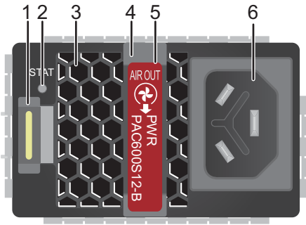
Figure 3-23 PAC600S12-B panel
