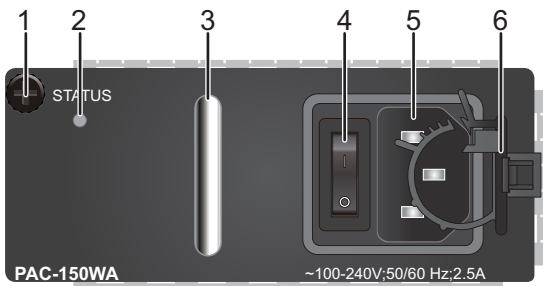
Figure 3-2 PAC-150WA panel
