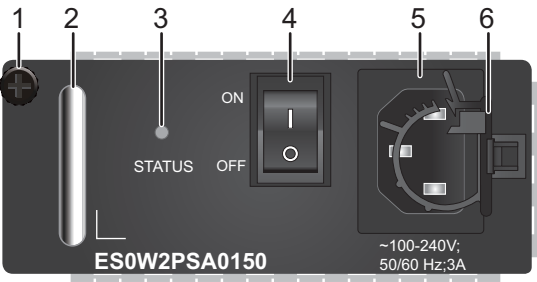
Figure 3-4 ES0W2PSA0150 panel
