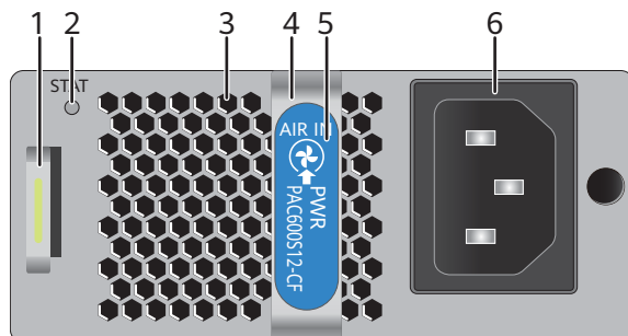
Figure 3-32 Panel of the PAC600S12-CF power module
