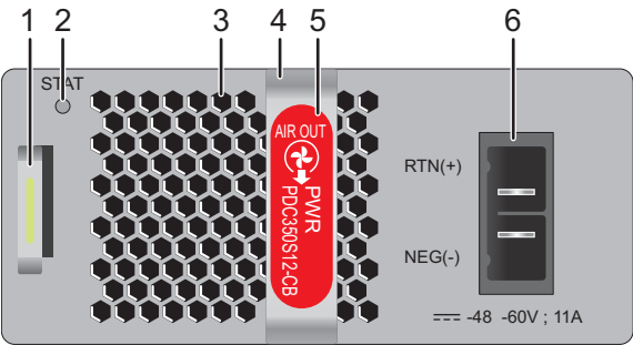
Figure 3-15 PDC350S12-CB panel
