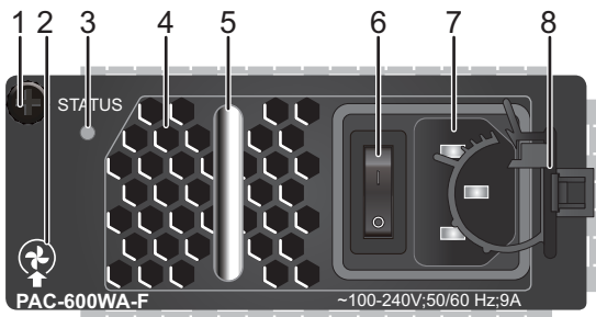
Figure 3-20 PAC-600WA-F panel
