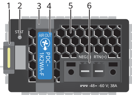
Figure 3-62 Panel of a PDC-1K2WA-F DC power module
