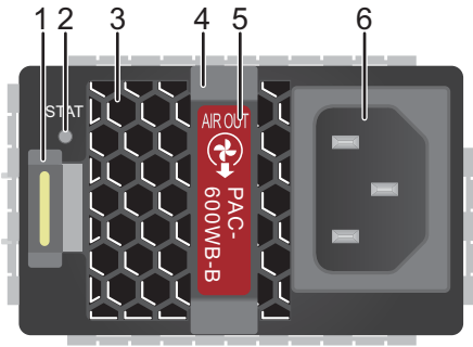
Figure 3-27 PAC-600WB-B panel
