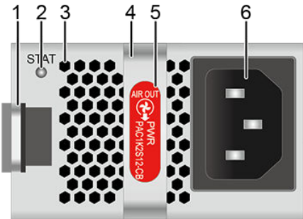
Figure 3-50 PAC1K2S12-CB panel
