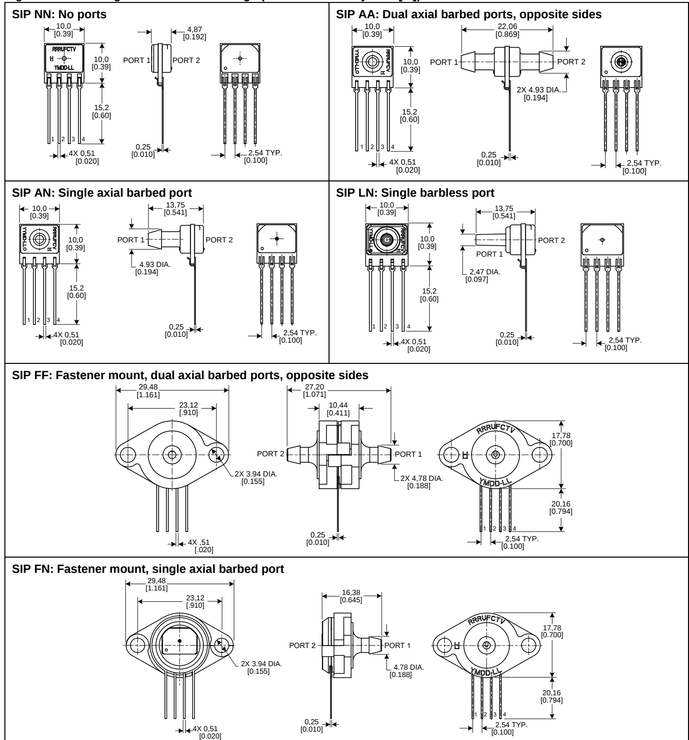
Figure 8. SIP Package Dimensional Drawings (For reference only: mm [in])
