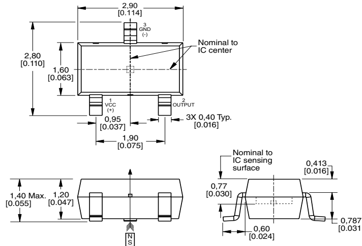
Figure 4. Mounting Dimensions (For reference only. mm/[in.] )
