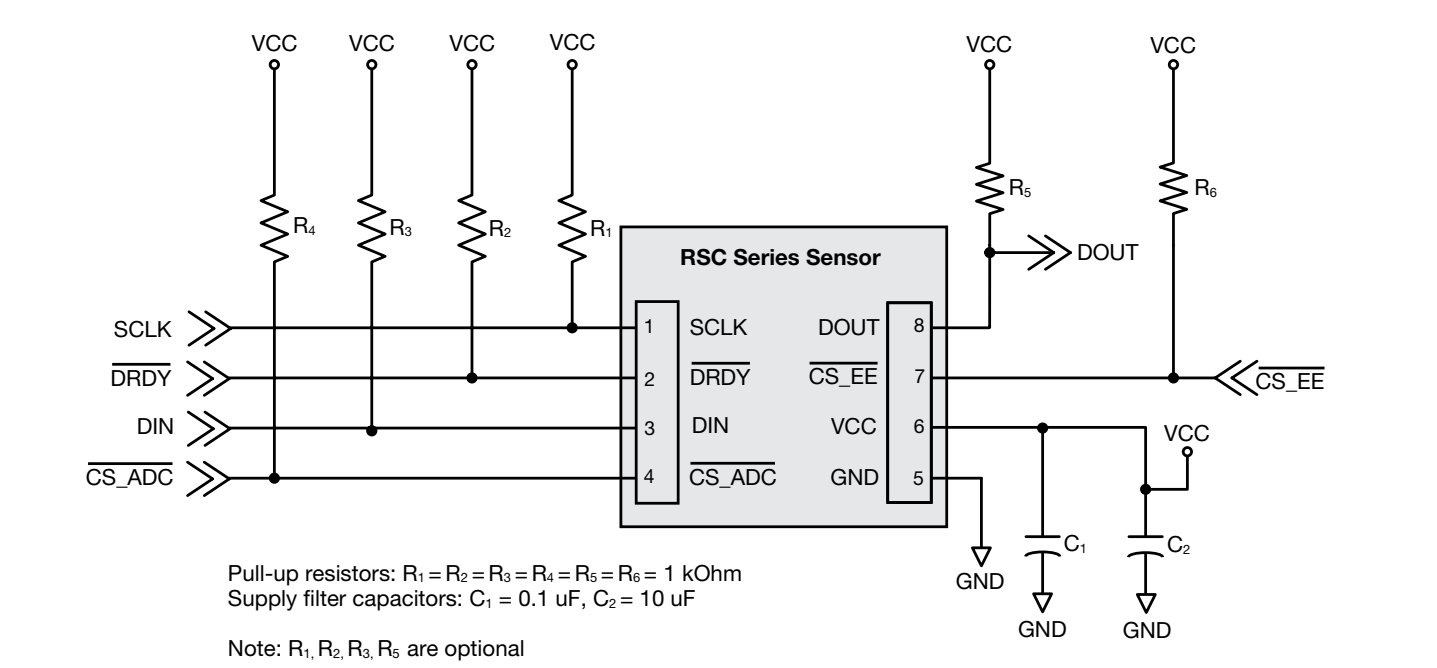
Figure 7. Recommended Circuit
