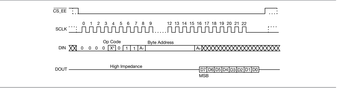
Figure 2-1. EEPROM Communications
