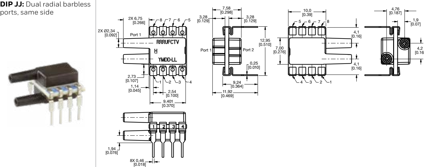
Figure 4. DIP Package Dimensional Drawings (continued)
