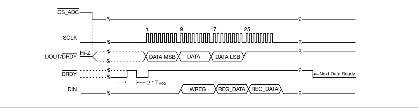
Figure 3-1. ADC Communciations and Initialization
