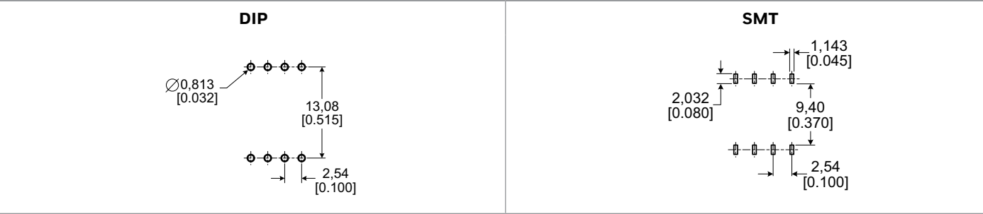
Figure 6. Recommended PCB Pad Layouts
