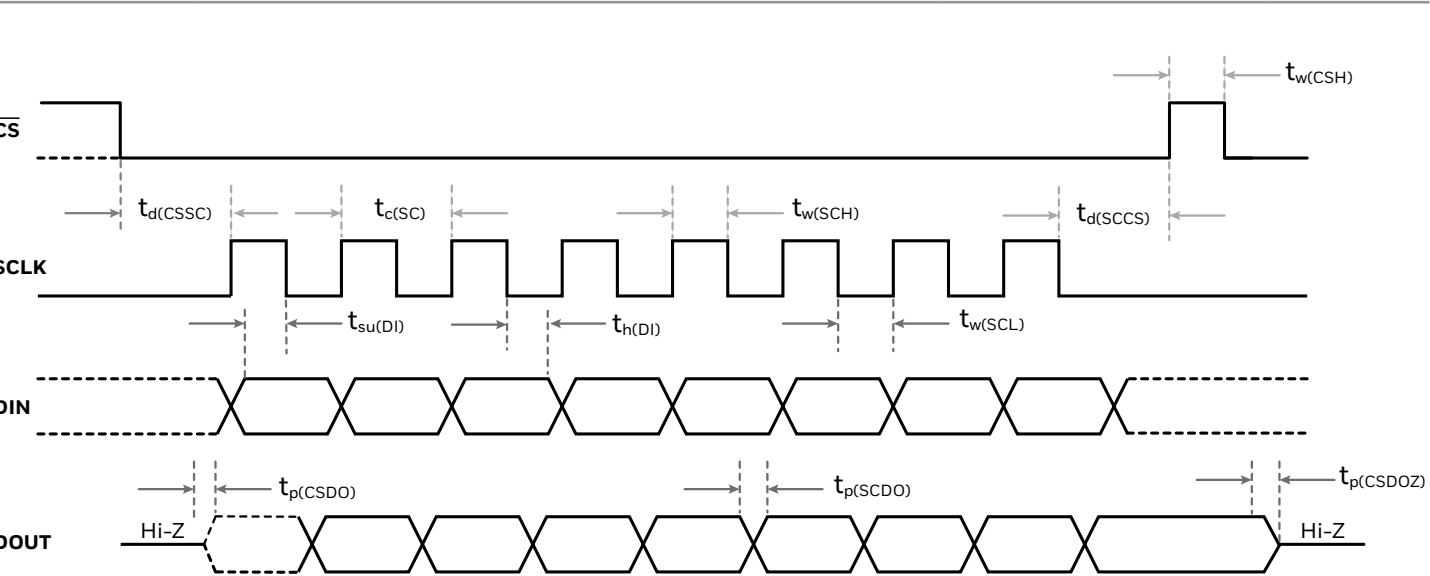
Figure 2. SPI Timing Requirements 1
