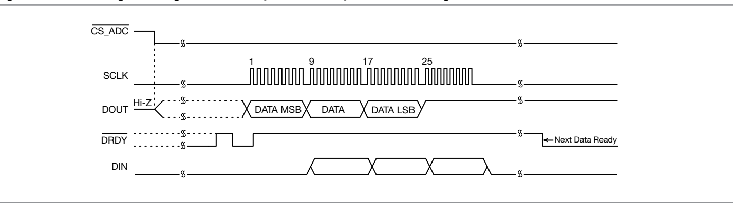
Figure 3-2. ADC Programming and Read Sequence – Temperature Reading
