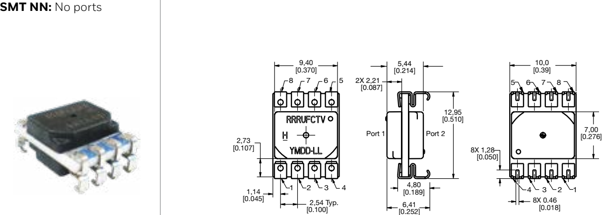
Figure 5. SMT Package Dimensional Drawings (For reference only: mm [in].)
