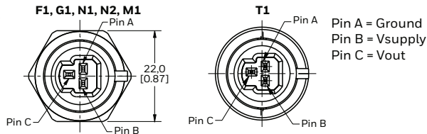
Figure 6. Metri-Pack Mounting Dimensions (For reference only. mm/[in].)
