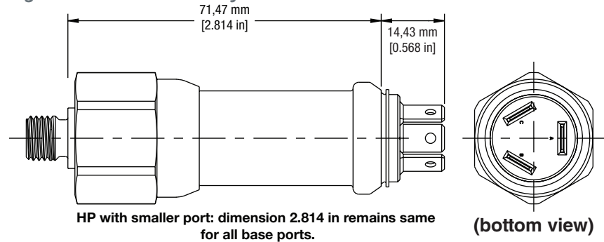
Figure 6. HP Series Base Style B
