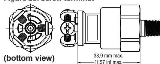
Figure 19. Screw terminal
