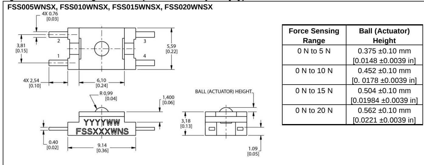
Figure 2. Sensor Mounting Dimensions (For reference only: mm/[in].)
