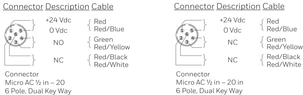
Figure 4. FFS Series Quick Disconnect Pinout
