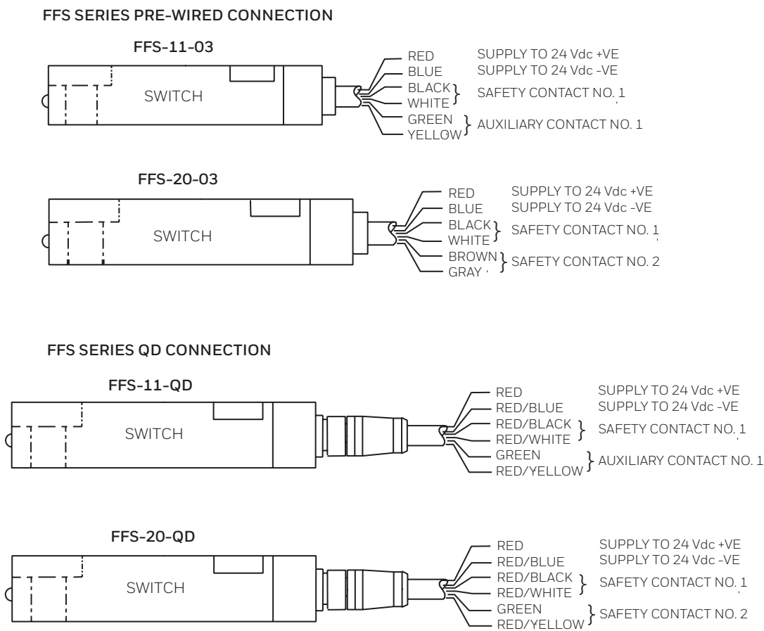
Figure 3. FFS Series Connections
