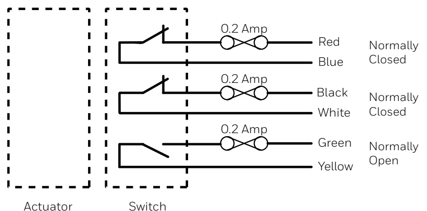
Figure 2. FF5 Wiring
