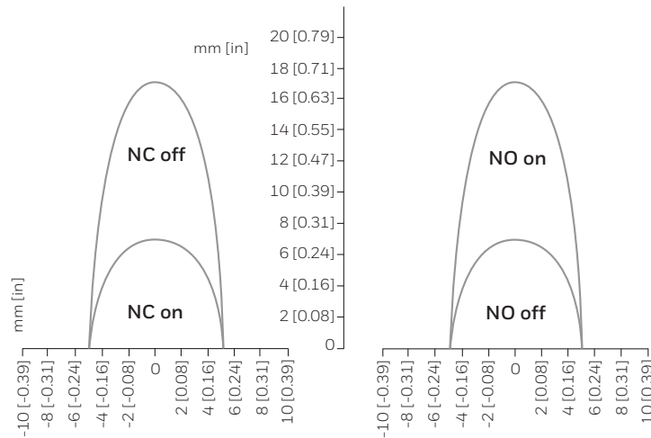
Figure 3. FF5 Series Sensing Distance
