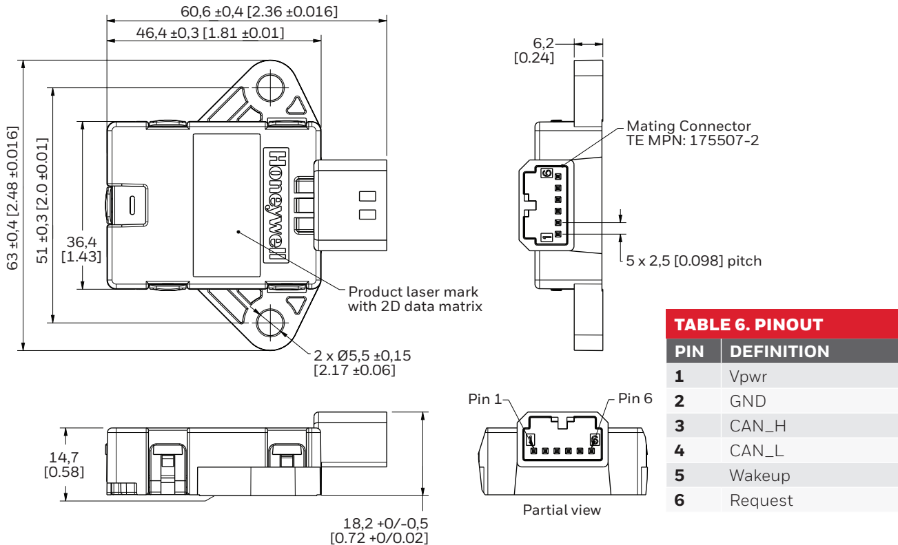
Figure 8. Mounting Dimensions (For reference only)
