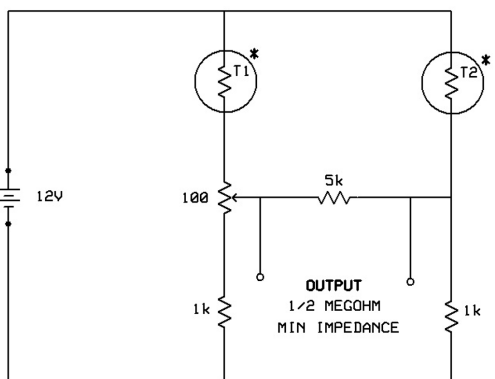
Figure 3. Typical Thermistors Thermal Conductivity Measurement Circuit
