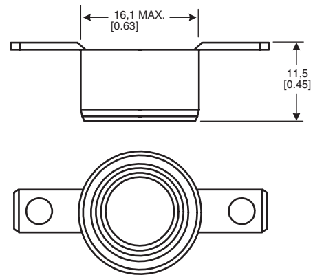
SERIES NAME 2450R Fully Sealed Thermostat
