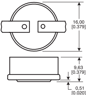
SERIES NAME 3450RC Ceramic “One-shot” ½ in Thermostat
