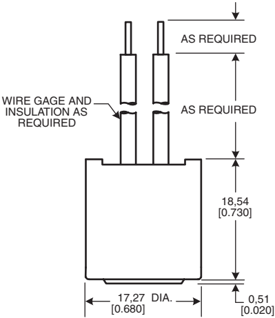
SERIES NAME 3455RBV Overmolded Automatic Reset Thermostat
