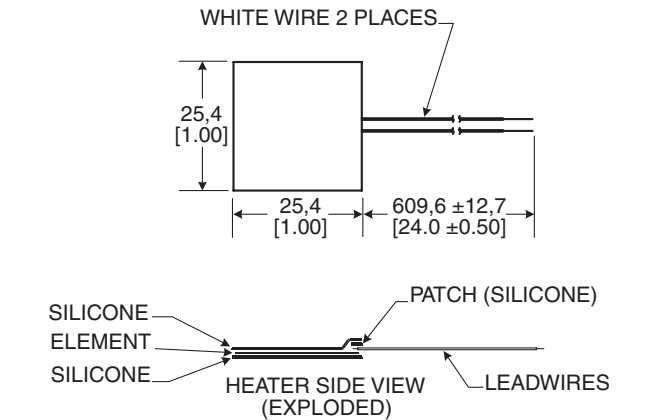
SERIES NAME 3200 Silicone Chemically etched Heater
