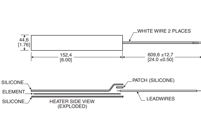
SERIES NAME 3100 Silicone Wire-wound Heater
