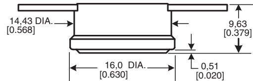
SERIES NAME 2450R Phenolic "One-shot" ½ in Thermostat
