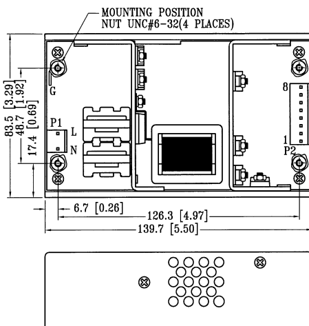
U-Bracket FORMAT
