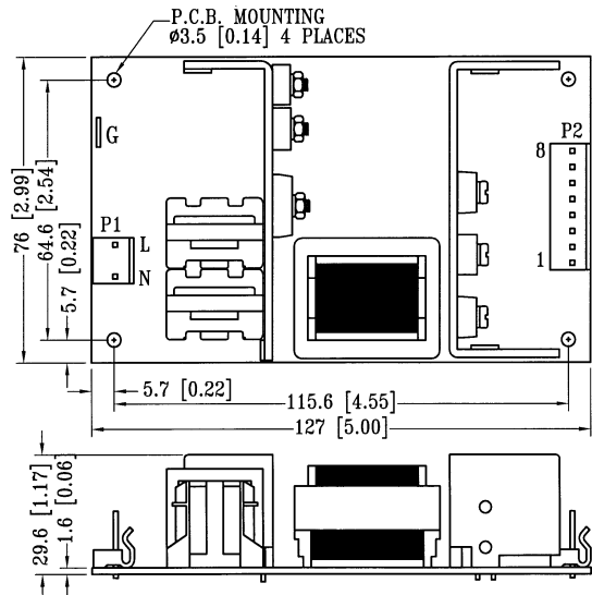
PCB FORMAT
