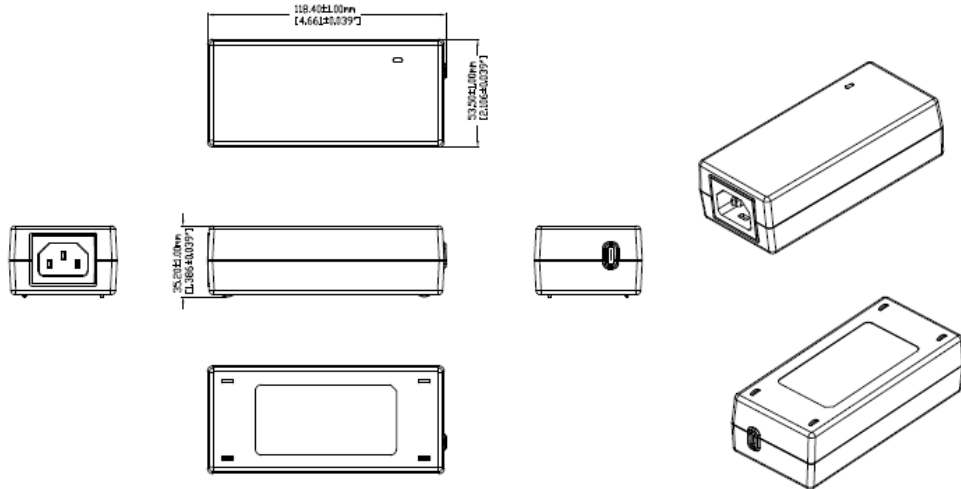
Drawing above is model with integrated USBC connector (suffix -RA)
