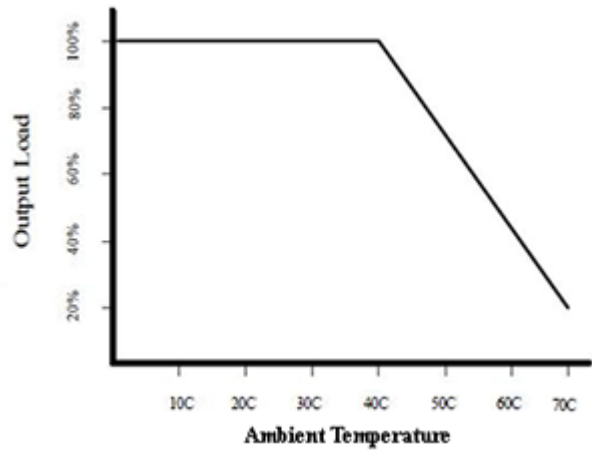
DERATING CURVE
