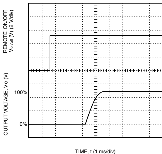
Figure 6. LW016AJ, BK, CL Typical Output Voltage Start-Up when Signal Applied to Remote On/Off
