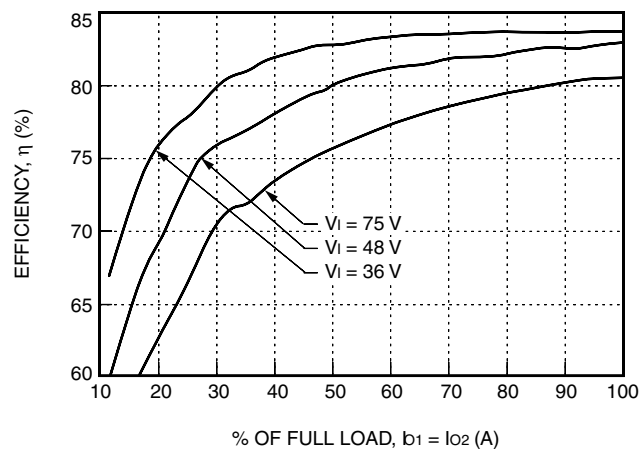
Figure 5. LW016CL Typical Converter Efficiency vs. Output Current
