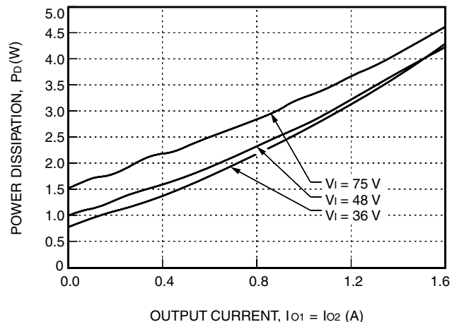
Figure 13. LW016AJ Power Dissipation vs. Output Current, T_A = 25 °C
