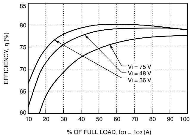
Figure 3. LW016AJ Typical Converter Efficiency vs. Output Current
