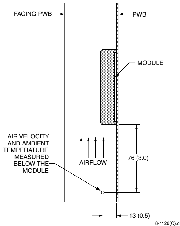
Figure 16. Experimental Test Setup
