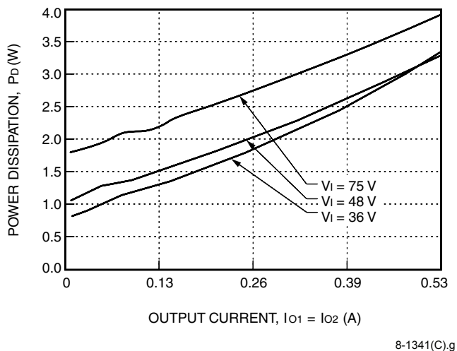
Figure 15. LW016CL Power Dissipation vs. Output Current, T_A = 25^\circ\text{C}
