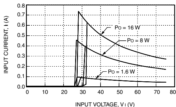
Figure 1. LW016AJ, BK, CL Typical Input Characteristics
