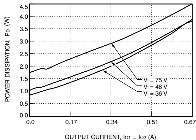
Figure 14. LW016BK Power Dissipation vs. Output Current, T_A = 25 °C
