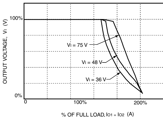
Figure 2. LW016AJ, BK, CL Typical Output Characteristics
