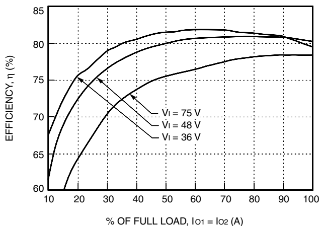
Figure 4. LW016BK Typical Converter Efficiency vs. Output Current
