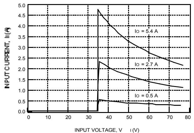
Figure 4. Typical JW150R Input Characteristics at Room Temperature
