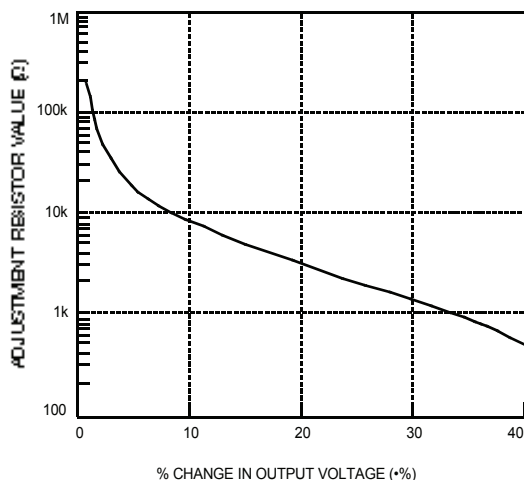
Figure 32. Resistor Selection for Decreased Output Voltage
