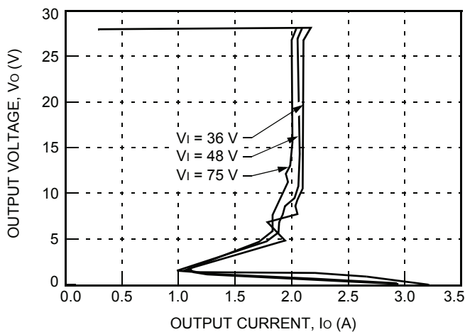
Figure 5. Typical JW050R Output Characteristics at Room Temperature
