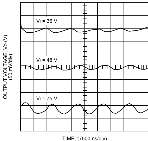
Figure 13. Typical JW050R Output Ripple Voltage at Room Temperature, 36 Vdc to 75 V Input, and 2.7 A Output
