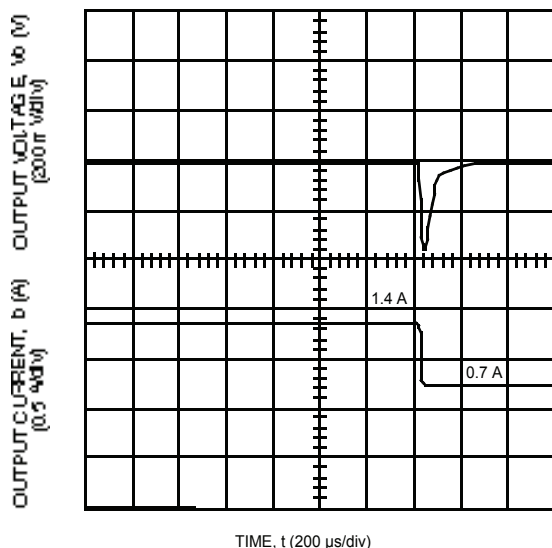
Figure 17. Typical JW050R Transient Response to Step Decrease in Load from 50% to 25% of Full Load at Room Temperature and 48 Vdc Input (Waveform Averaged to Eliminate Ripple Component.)
