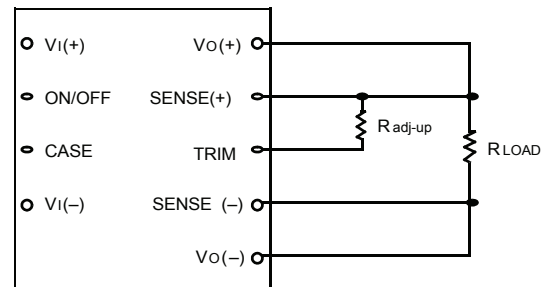
Figure 33. Circuit Configuration to Increase Output Voltage
