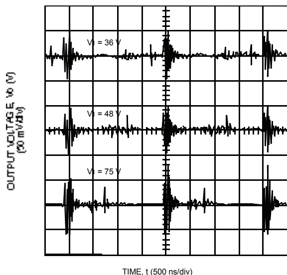
Figure 14. Typical JW075R Output Ripple Voltage at Room Temperature, 36 Vdc to 75 V Input, and 2.7 A Output
