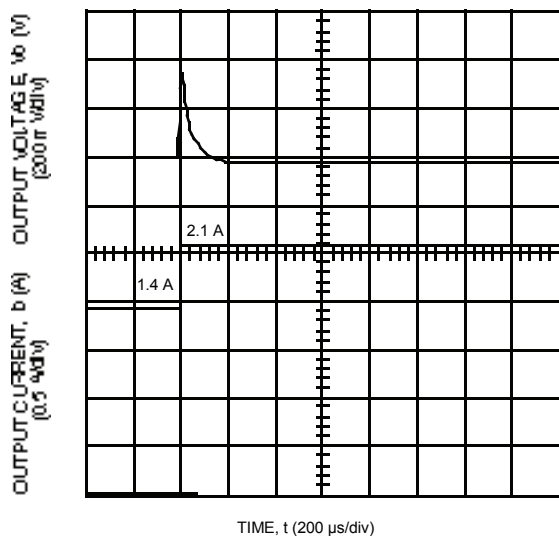
Figure 21. Typical JW050R Transient Response to Step Increase in Load from 50% to 75% of Full Load at Room Temperature and 48 Vdc Input (Waveform Averaged to Eliminate Ripple Component.)
