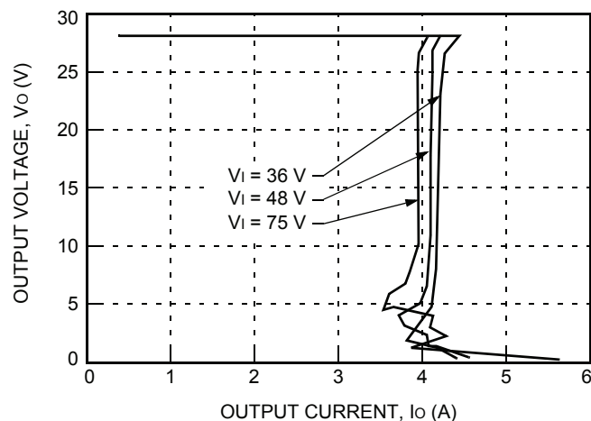
Figure 7. Typical JW100R Output Characteristics at Room Temperature
