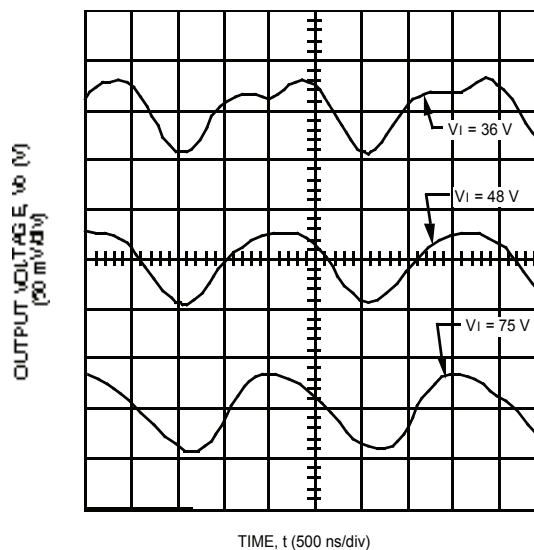
Figure 16. Typical JW150R Output Ripple Voltage at Room Temperature, 36 Vdc to 75 V Input, and 5.4 A Output
