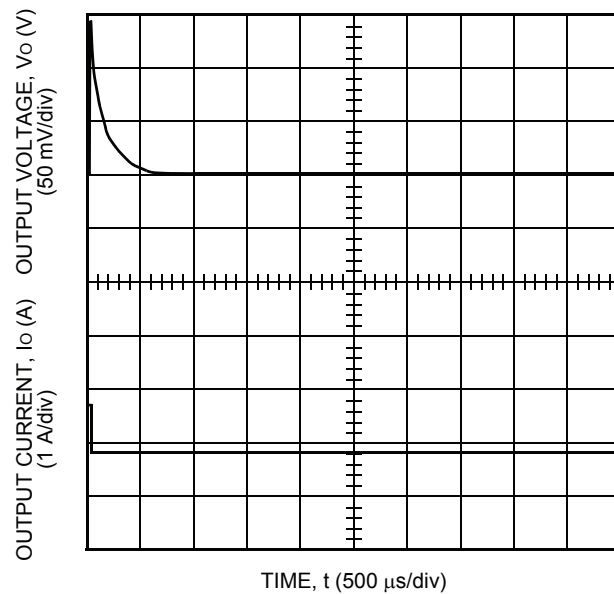
Figure 23. Typical JW100R Transient Response to Step Increase in Load from 50% to 75% of Full Load at Room Temperature and 48 Vdc Input (Waveform Averaged to Eliminate Ripple Component.)
