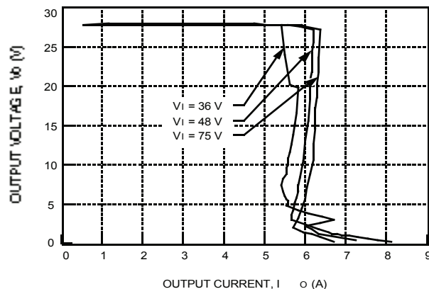
Figure 8. Typical JW150R Output Characteristics at Room Temperature
