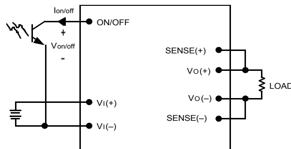
Figure 29. Remote On/Off Implementation
