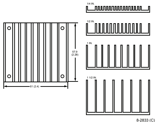
Figure 44. Transverse Heat Sink
