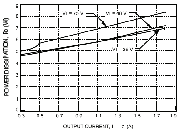
Figure 37. JW050R Power Dissipation vs. Output Current at 25 °C
