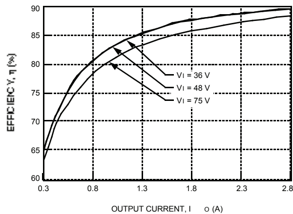
Figure 10. Typical JW075R Converter Efficiency vs. Output Current at Room Temperature
