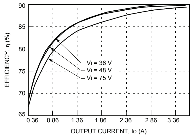
Figure 11. Typical JW100R Converter Efficiency vs. Output Current at Room Temperature
