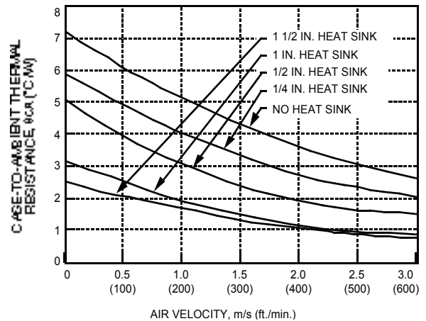
Figure 41. Case-to-Ambient Thermal Resistance Curves; Either Orientation
