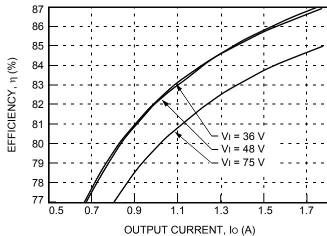
Figure 9. Typical JW050R Converter Efficiency vs. Output Current at Room Temperature
