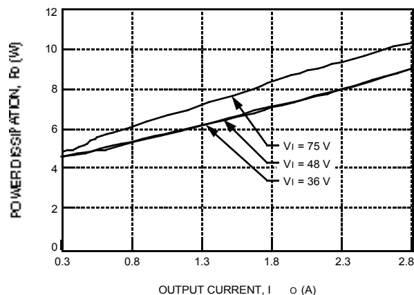
Figure 38. JW075R Power Dissipation vs. Output Current at 25 °C
