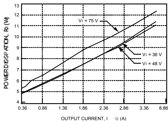
Figure 39. JW100R Power Dissipation vs. Output Current at 25 °C
