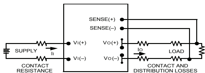
Figure 30. Effective Circuit Configuration for Single-Module Remote-Sense Operation
