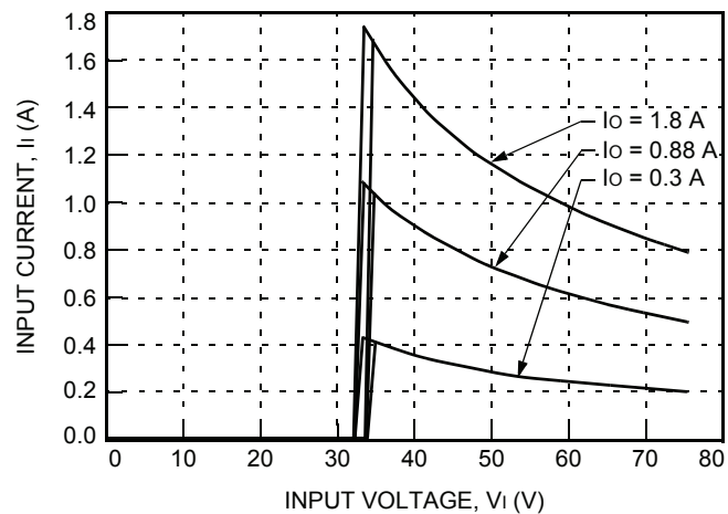
Figure 1. Typical JW050R Input Characteristics at Room Temperature
