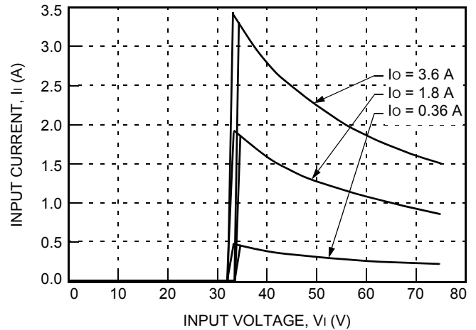
Figure 3. Typical JW100R Input Characteristics at Room Temperature
