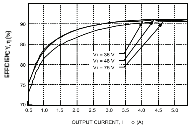
Figure 12. Typical JW150R Converter Efficiency vs. Output Current at Room Temperature
