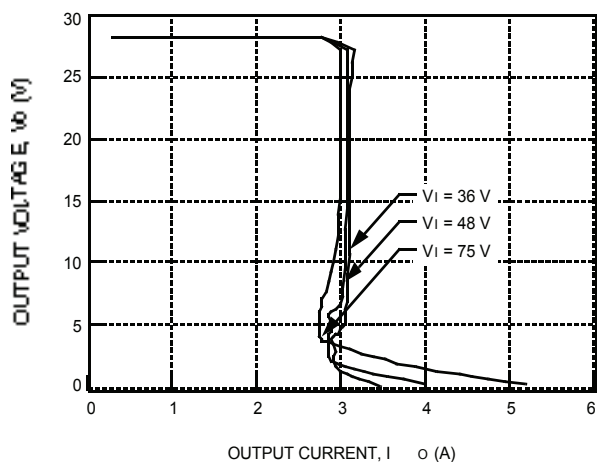
Figure 6. Typical JW075R Output Characteristics at Room Temperature
