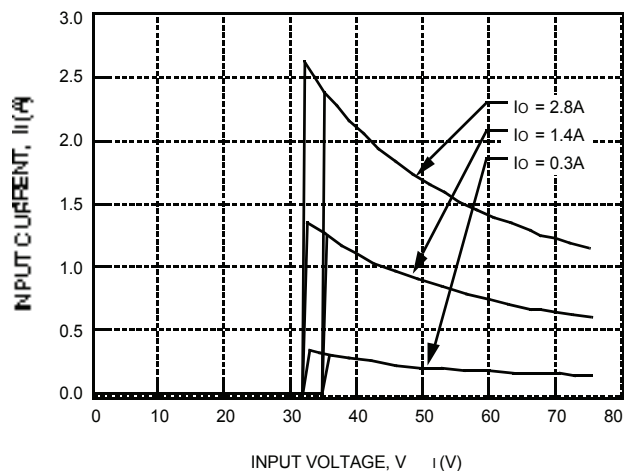
Figure 2. Typical JW075R Input Characteristics at Room Temperature
