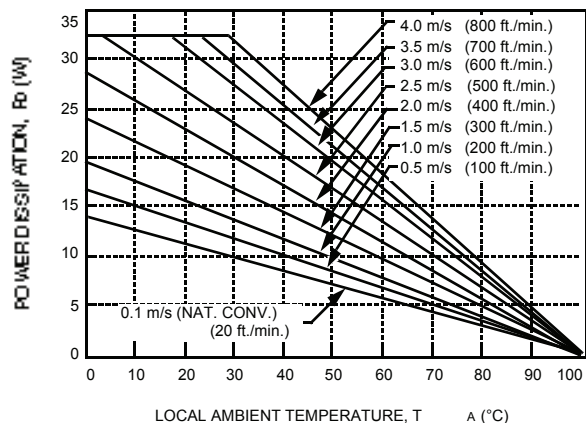
Figure 36. Forced Convection Power Derating with No Heat Sink; Either Orientation
