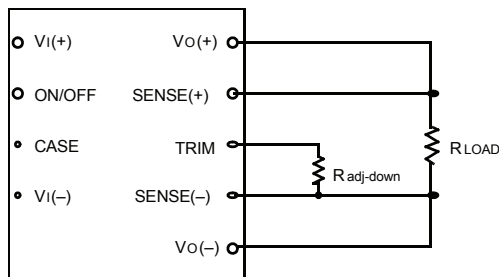
Figure 31. Circuit Configuration to Decrease Output Voltage
