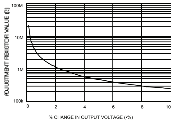
Figure 34. Resistor Selection for Increased Output Voltage
