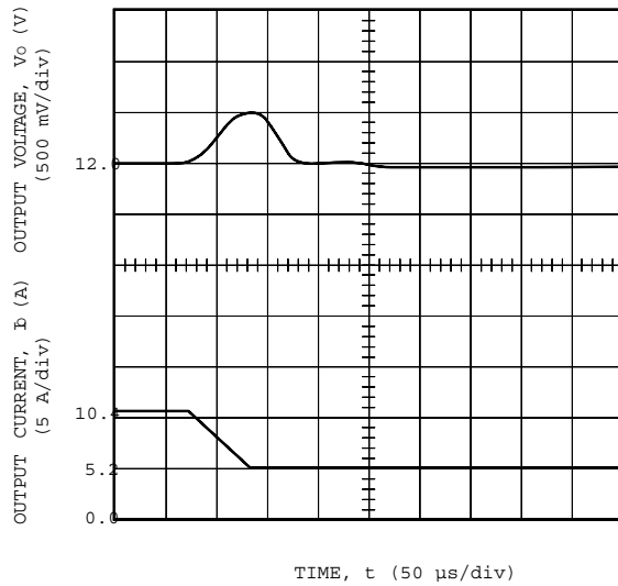
Figure 5. Typical FC250B1 Transient Response to Step Decrease in Load from 50% to 25% of Full Load at Room Temperature and 28 V Input (Waveform Averaged to Eliminate Ripple Component.)
