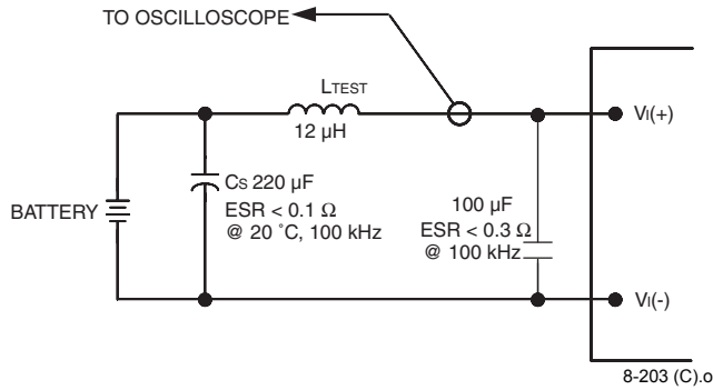
Figure 8. Input Reflected-Ripple Test Setup
