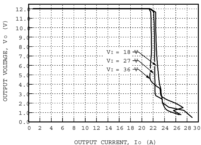
Figure 2. Typical FC250B1 Output Characteristics at Room Temperature
