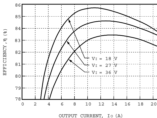
Figure 3. Typical FC250B1 Efficiency vs. Output Current at Room Temperature
