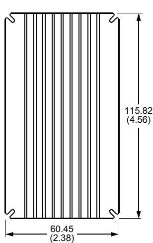
Figure 25.Longitudinal Heat Sink
