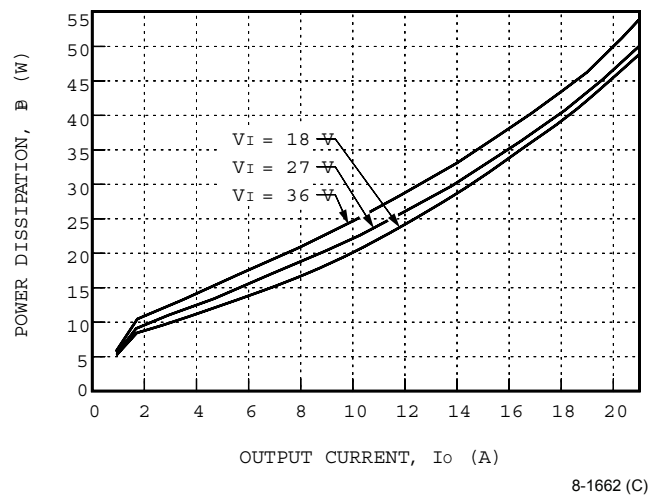
Figure 23. FC250B1 Power Dissipation vs. Output Current at 25 °C
