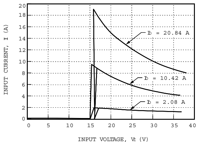
Figure 1. Typical FC250B1 Input Characteristics at Room Temperature
