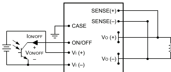
Figure 11. Remote On/Off Implementation
