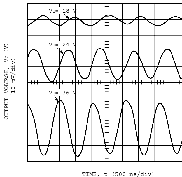
Figure 4. Typical FC250B1 Output Ripple Voltage at Room Temperature and Full Load Output
