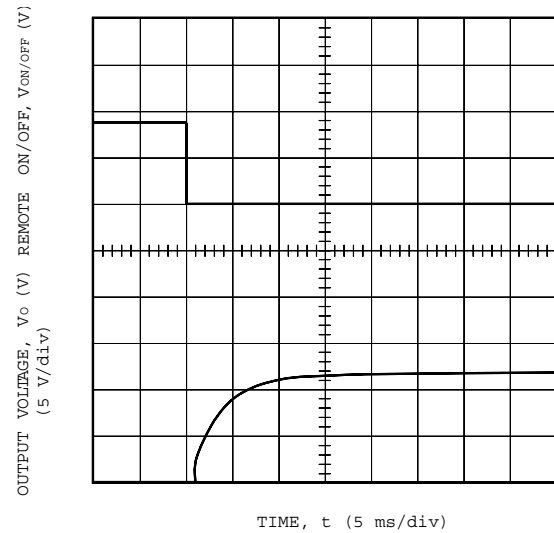
Figure 7. Typical FC250B1 Start-Up Transient at Room Temperature, 28 V Input
