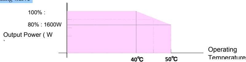
Thermal Derating Curve
