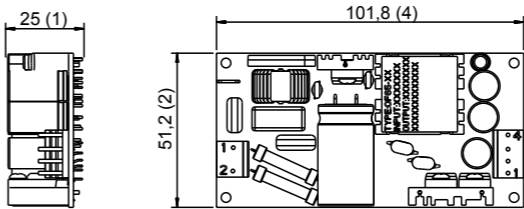
Alle Abmessungen in Millimeter (Inch), Abweichung ± 0,5 (0.02) All Dimensions in Millimeter (Inch), Deviation ± 0,5 (0.02)
