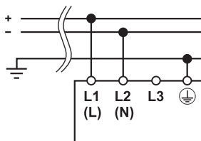
DC Line
