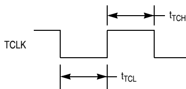
Figure 20-2. Timer Input Timing
