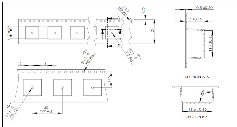
Figure 8: Tape dimensions and layout (All dimensions in millimeters)
