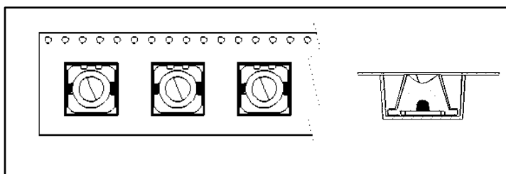
Figure 9: Orientation of lens in tape pockets
