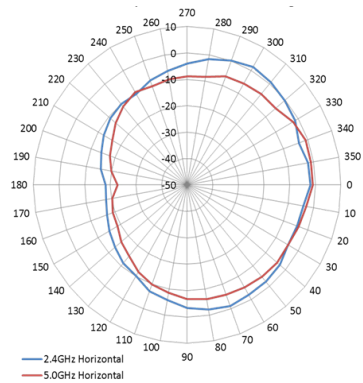
H-Plane Pattern with metal mounting plate
