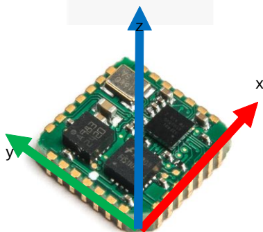
Figure 16. Default Sensor fixed Coordinate System for the FMT1000-Series Module
