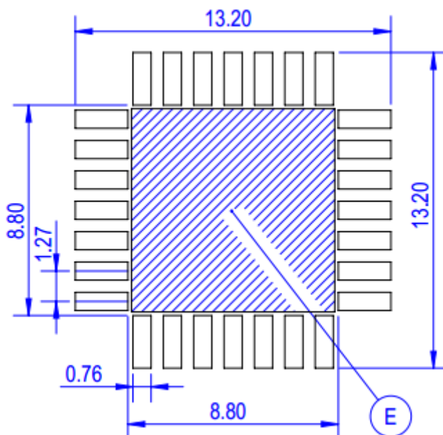
Figure 18. Land Pattern Recommendation
