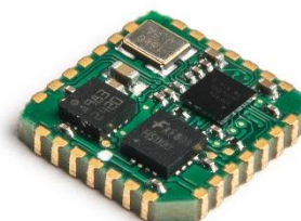
Figure 1. FMT1000-series Module
