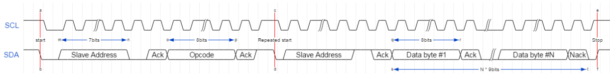
Figure 7. Read Message Transfer using a Repeated Start (I 2 C)
