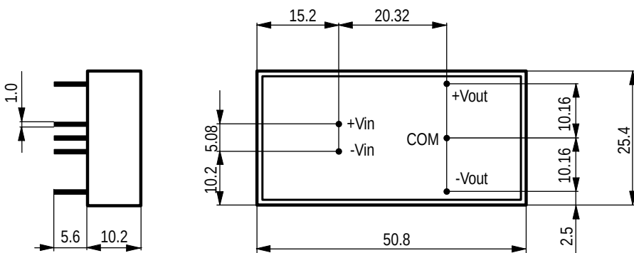
UCW 10 Watt Series Dual Output Models View from bottom
