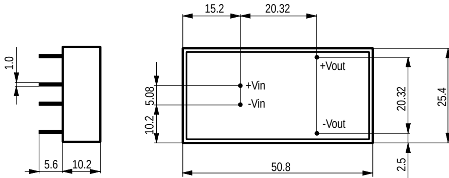
UCW 10 Watt Series Single Output Models View from bottom
