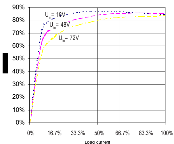
Efficiency (typical ECU48-1575, U_{in} = 18-72Vdc )
