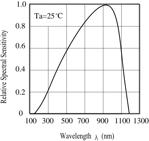
Fig.1 Spectral Sensitivity
