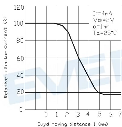
Fig.2 Relative Collector Current vs. Card Moving Distance (1)
