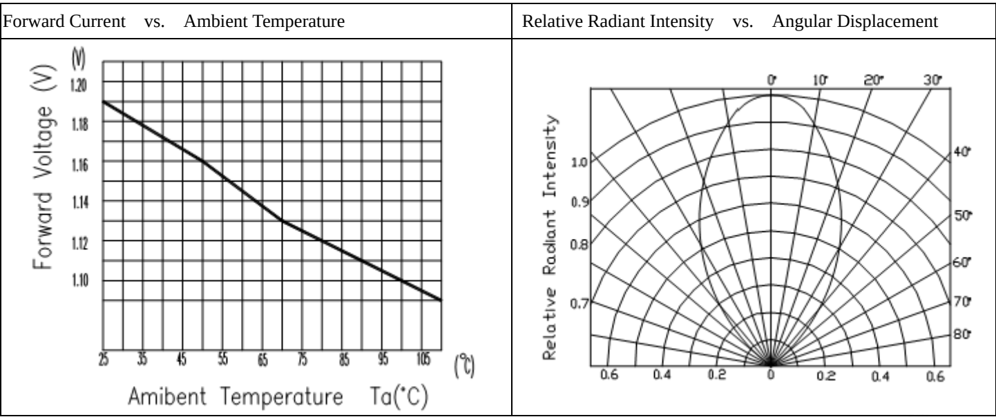
Typical Electro/Optical/Characteristics Curves for PT
