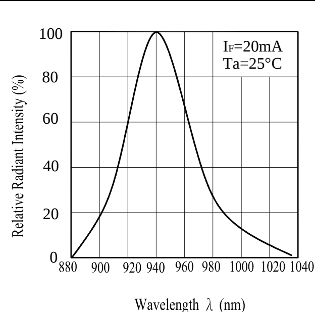
Spectral Sensitivity
