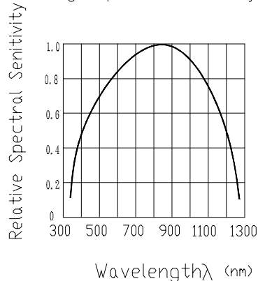
Fig.5 Spectral Sensitivity
