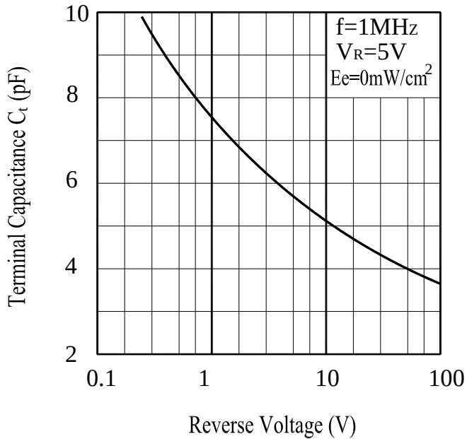
Fig.5 Terminal Capacitance vs. Reverse Voltage
