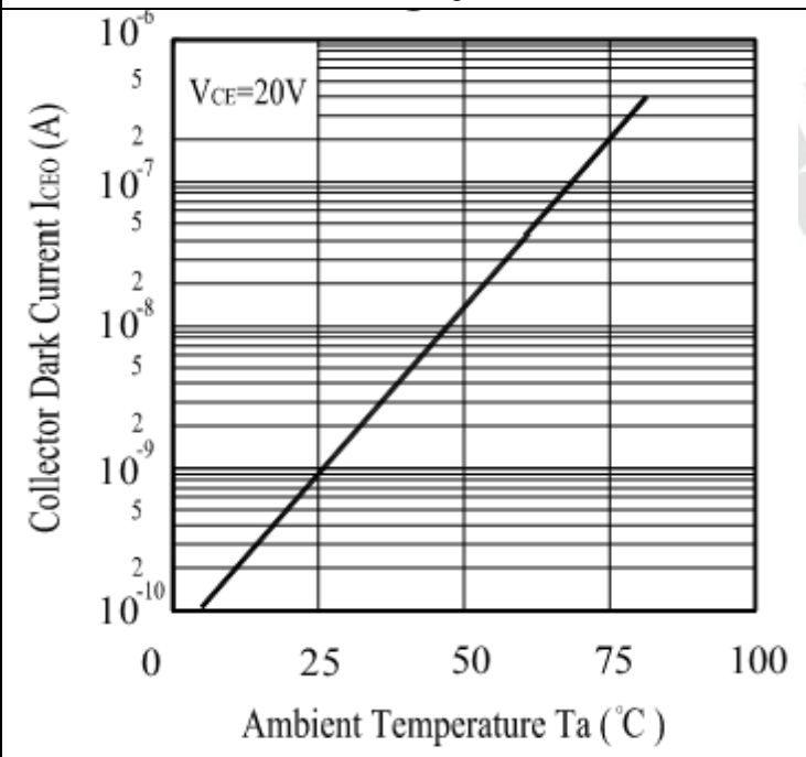
Collector Current vs. Ambient Temperature
