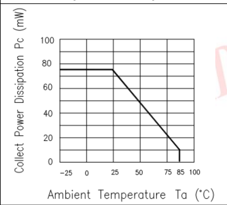
Collector Power Dissipation vs. Ambient Temperature
