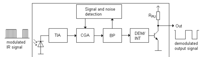
Block Diagram
